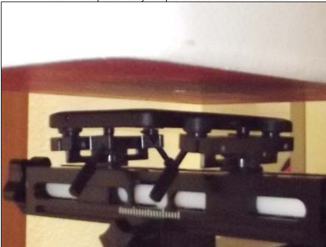
Photo 12: Test position body worn front side with 15 mm distance
