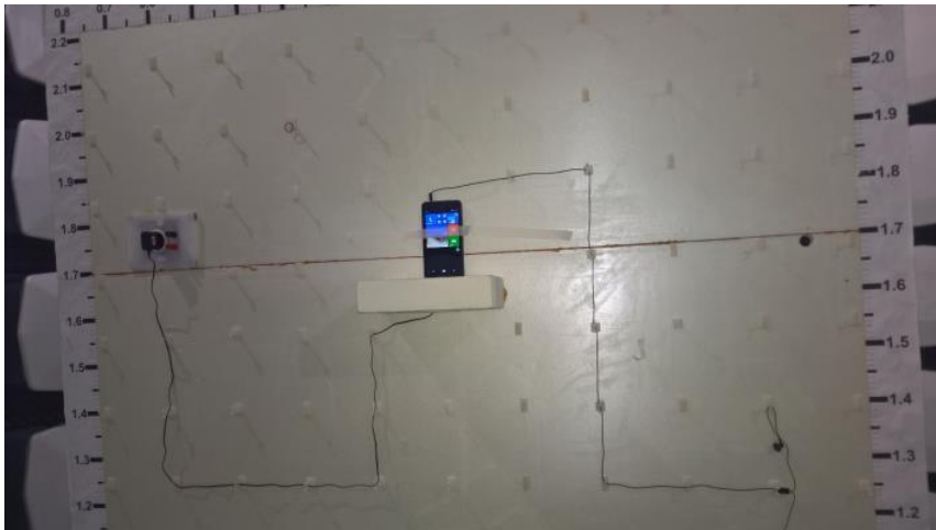
Picture 1. FCC Part 15C Radiated emissions
