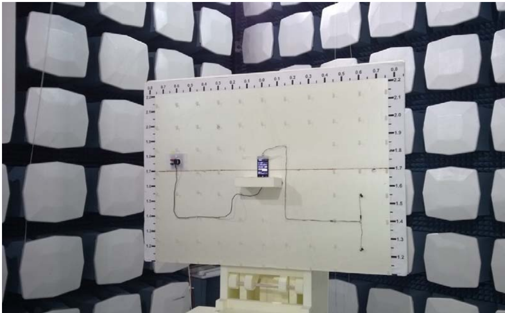
Picture 1. FCC Part 15C Radiated emissions
