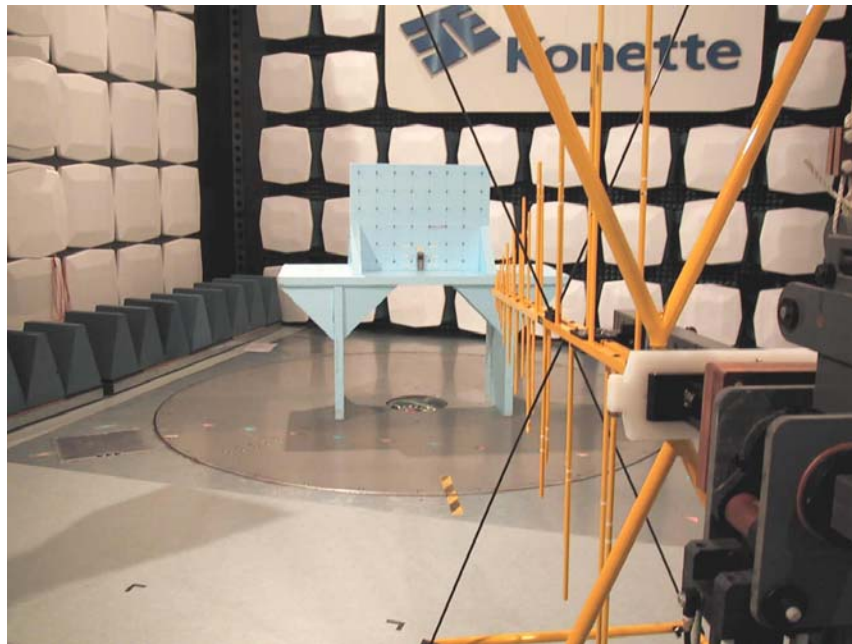
Picture 1: Test setup for radiated RF output power and spurious emission test below 3 GHz frequency, EUT in vertical orientation
