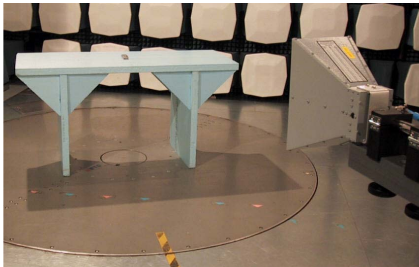
Picture 2: Test setup for spurious emission test over 3 GHz frequency, EUT in horizontal orientation
