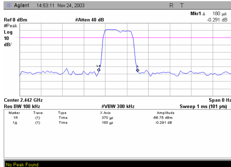
Picture 9: Duration of one transmission during paging cycle, channel 40
