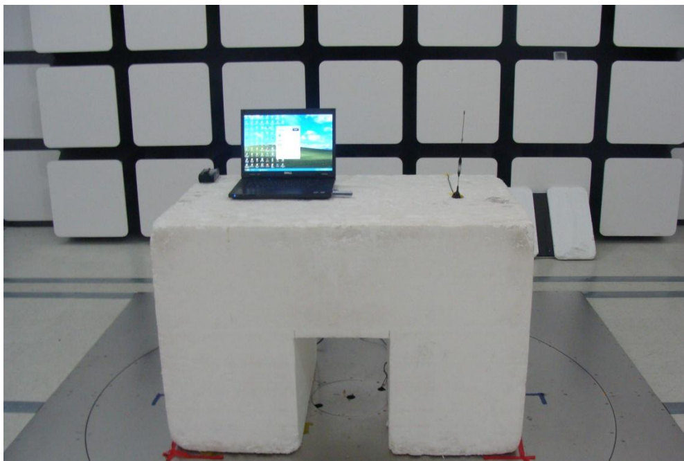
EUT Link without USB Cable
