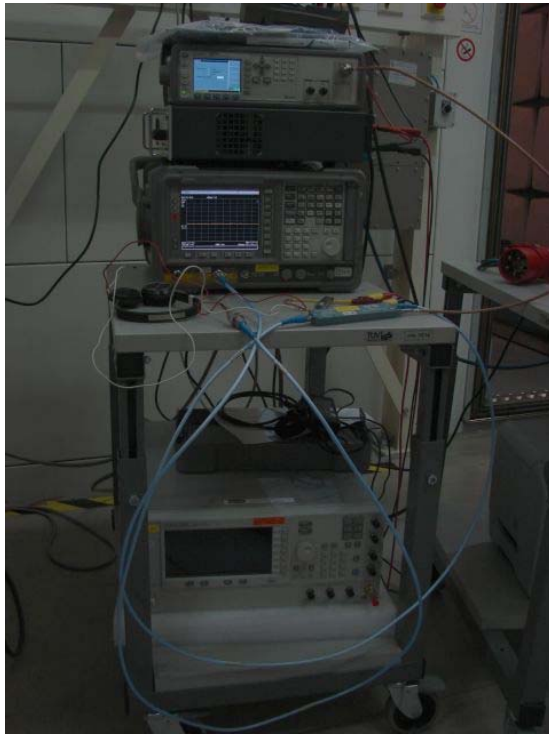
Picture 1: Conducted measurement test setup
