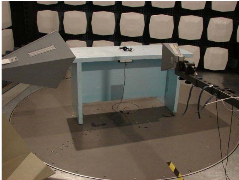
Picture 3: Radiated emission test setup 1 GHz – 18 GHz
