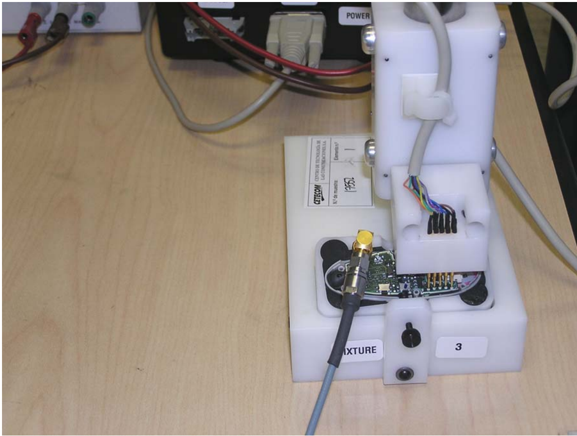
Test setup – EUT in test fixture
