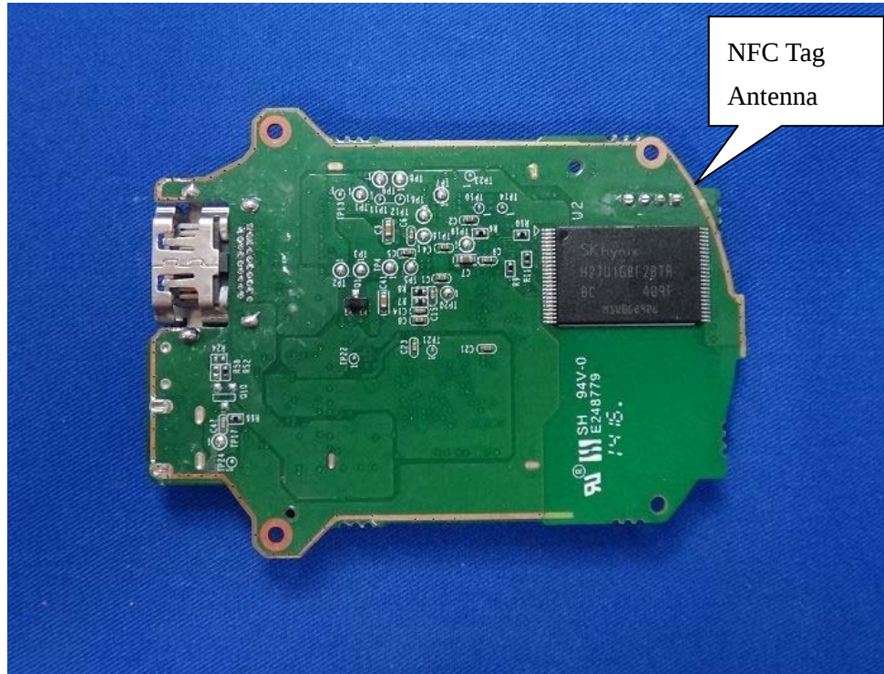
(11) EUT Photo
