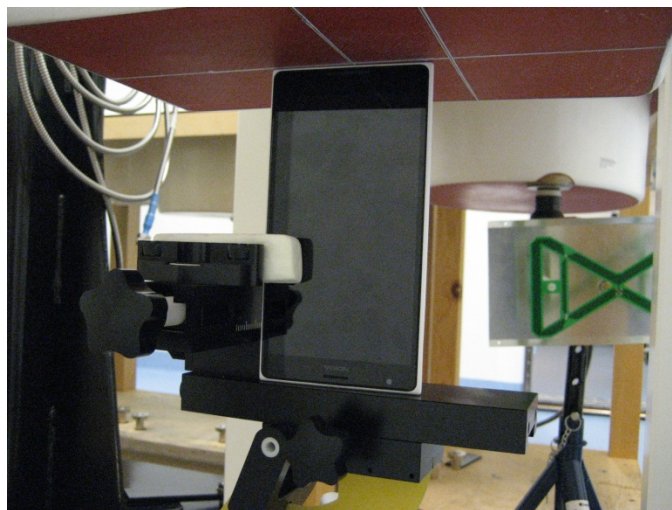
Photo of the device positioned for 10g Extremity measurement – bottom edge facing phantom.
