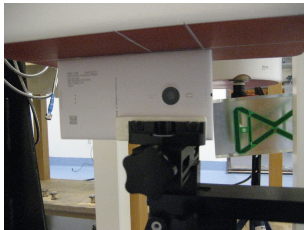
Photo of the device positioned for 10g Extremity measurement – right edge facing phantom.
