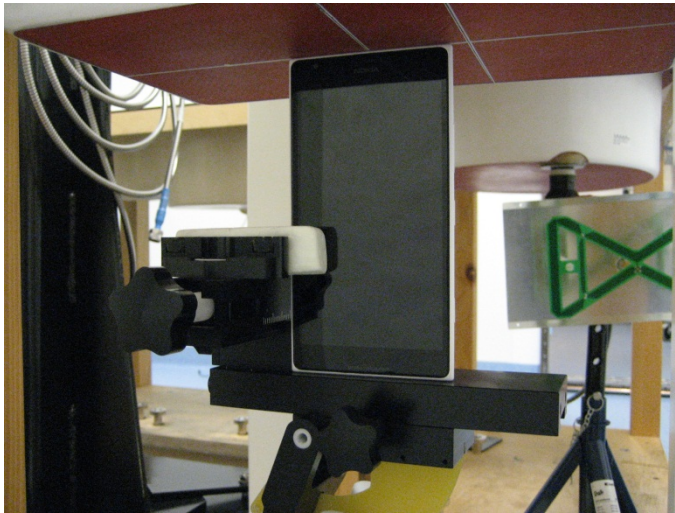
Photo of the device positioned for 10g Extremity measurement – top edge facing phantom.
