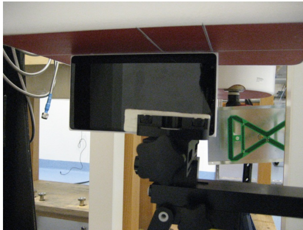
Photo of the device positioned for 10g Extremity measurement – left edge facing phantom.
