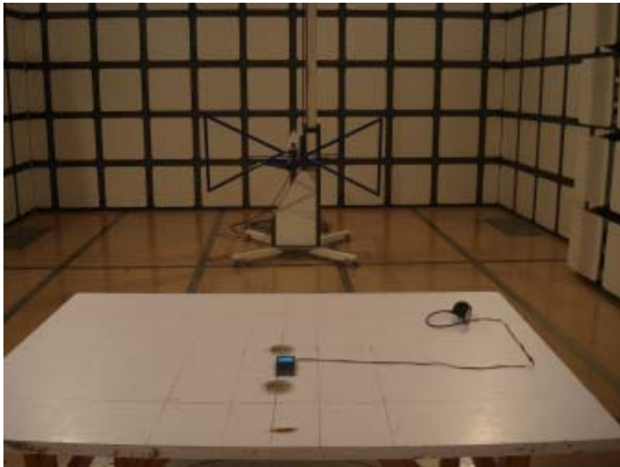
(4) Radiated Emission Test Setup Photo
