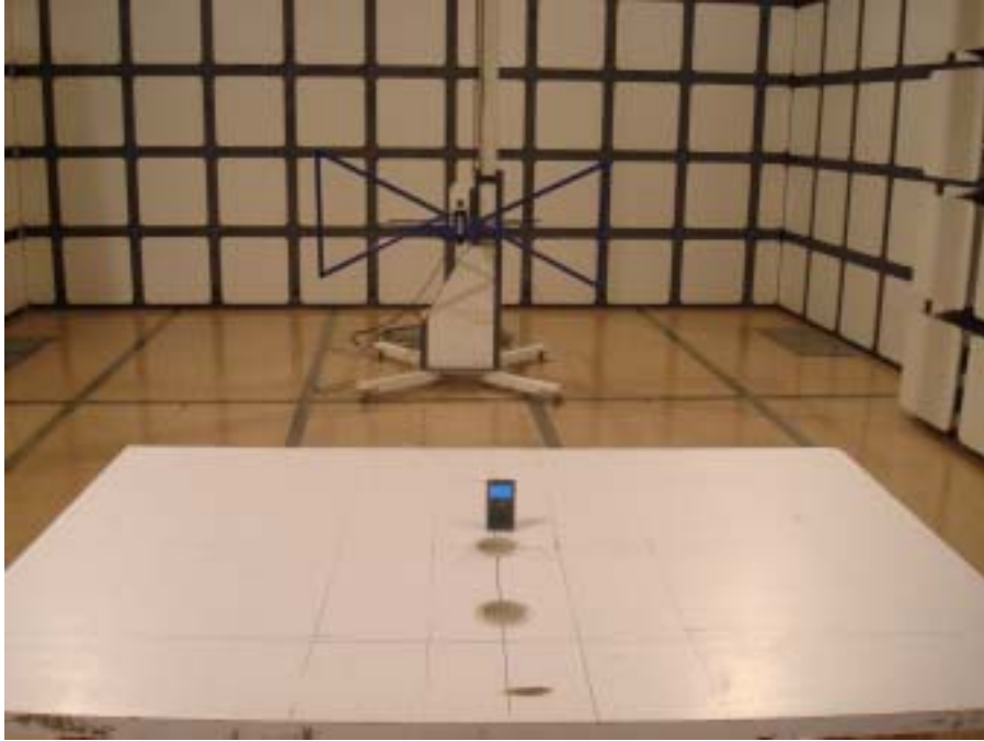
(3) Radiated Emission Test Setup Photo
