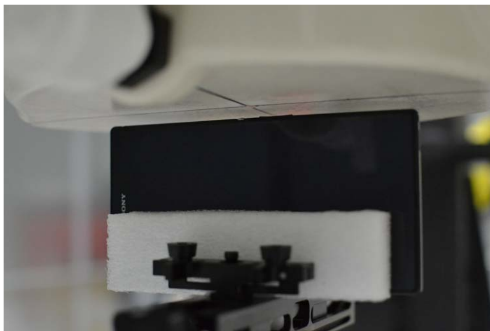
SAR Test Setup Photo 7 – Right Edge at 5 mm
