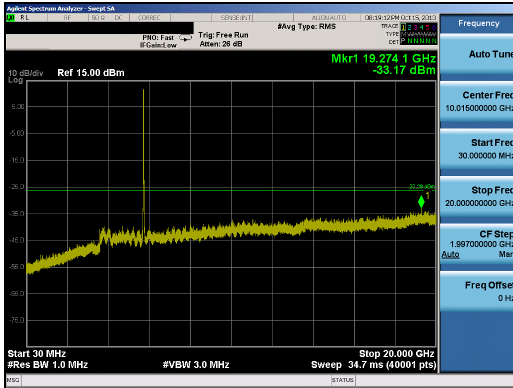
Plot 6-57. Conducted Spurious Plot (802.11a – Ch. 149)
