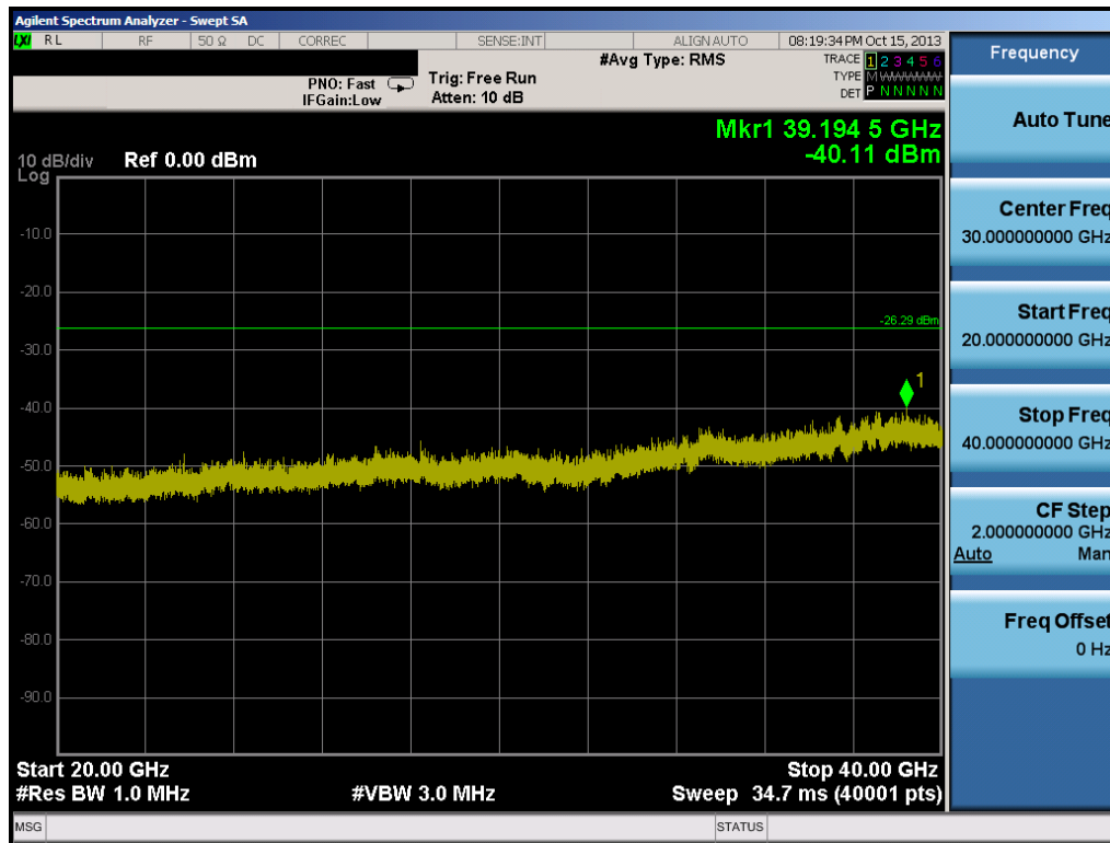
Plot 6-58. Conducted Spurious Plot (802.11a – Ch. 149)
