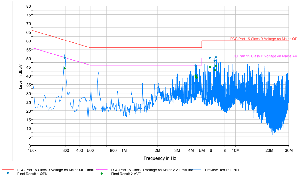
Plot 6-73. Line Conducted Plot with 802.11a (L1)
