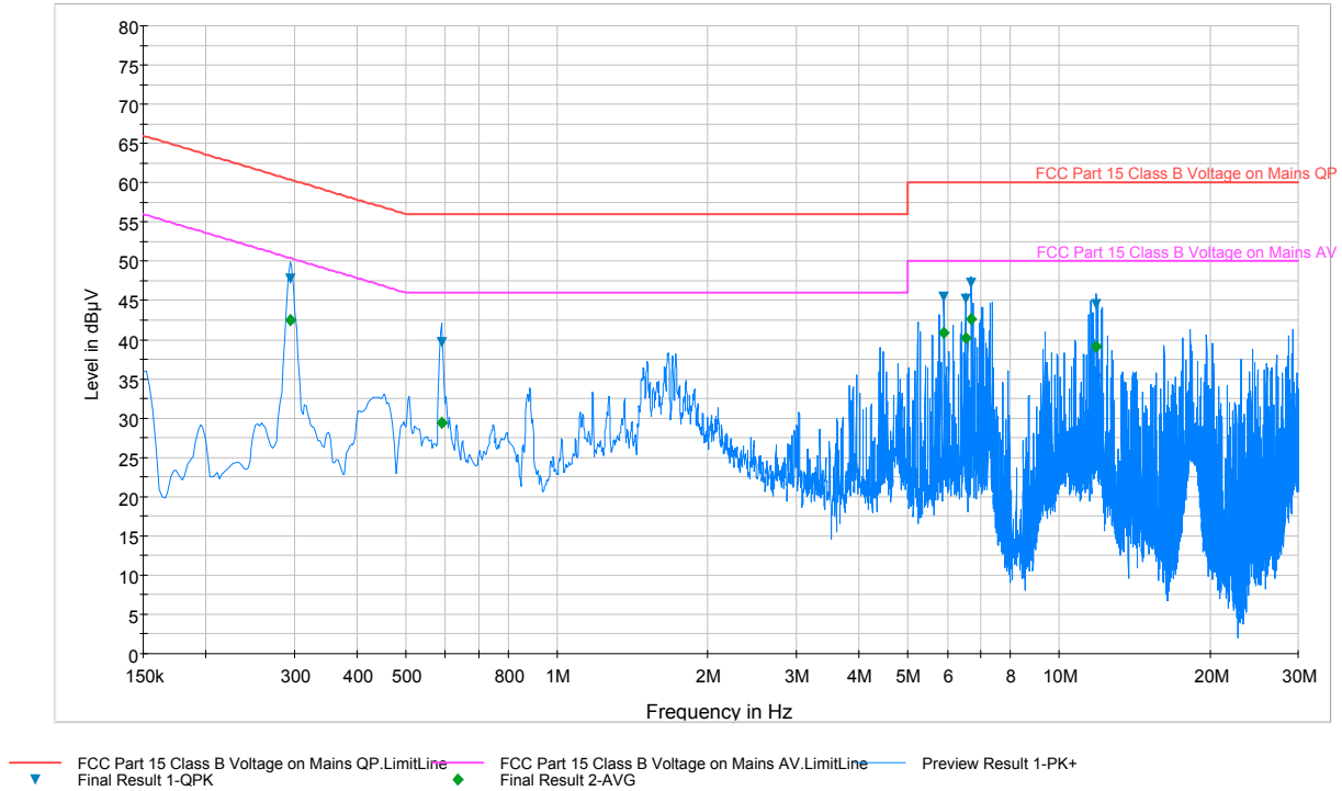
Plot 6-74. Line Conducted Plot with 802.11a (N)
