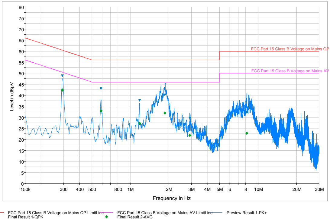
Plot 6-71. Line Conducted Plot with 802.11b (L1)
