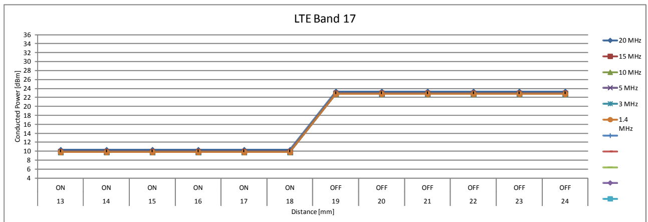
Top Edge position, Sensor 2 active, moving downward
