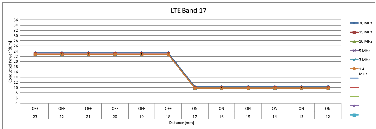
Top Edge position, Sensor 2 active, moving upward
