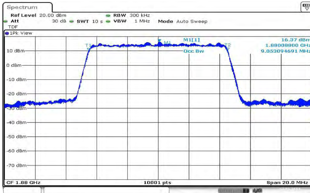
Plot 4: 10 MHz (99% - OBW)
