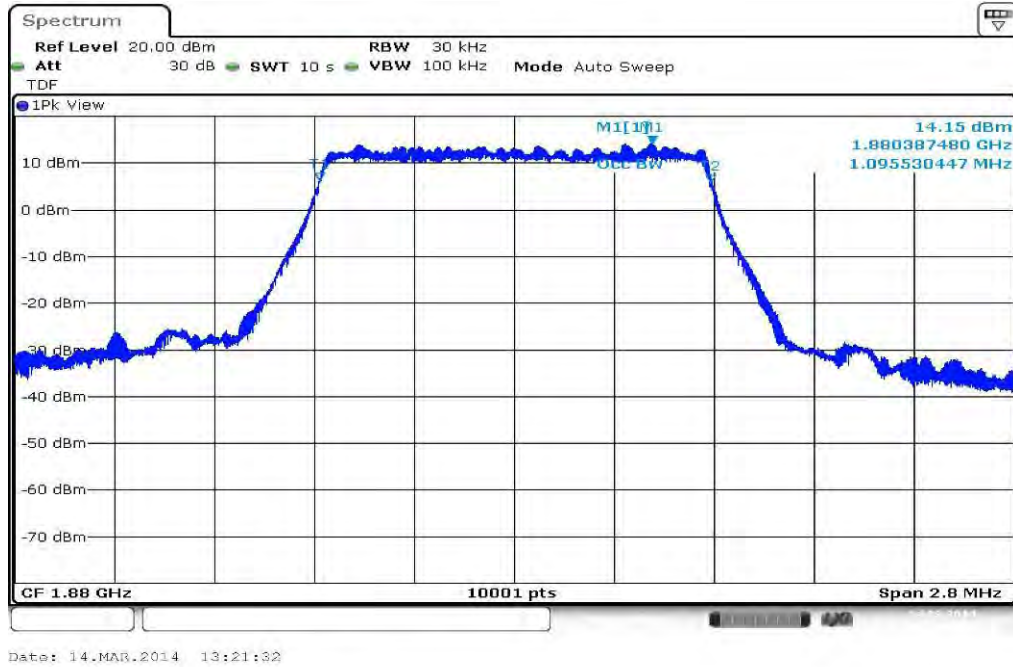
Plot 1: 1.4 MHz (99% - OBW)
