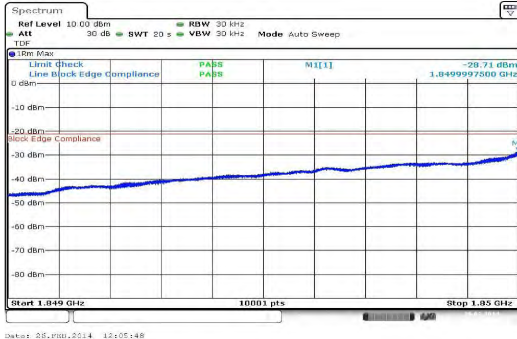
Plot 3: Lowest channel – 16-QAM
