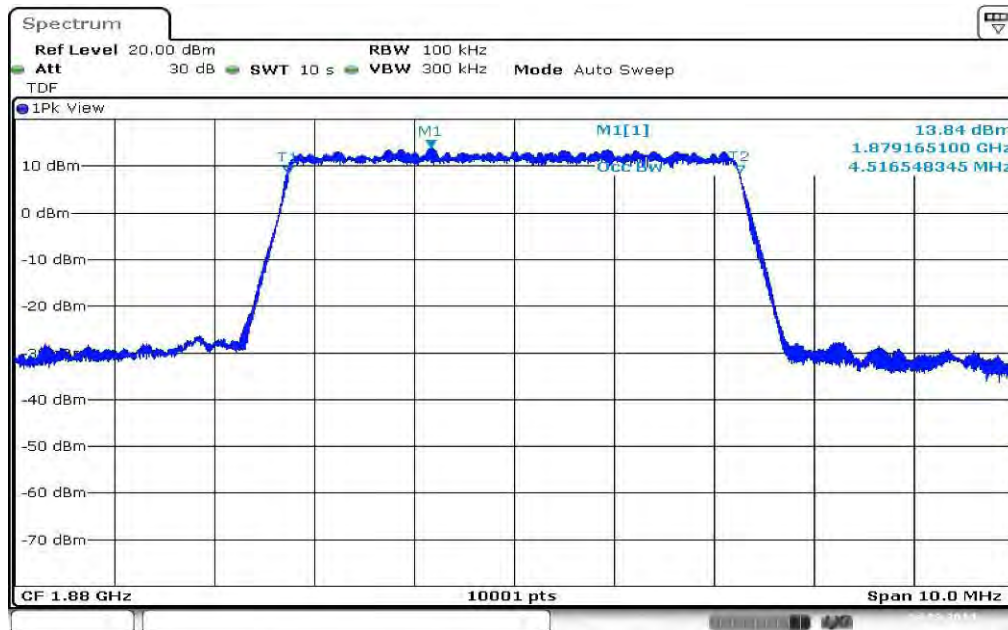
Plot 3: 5 MHz (99% - OBW)
