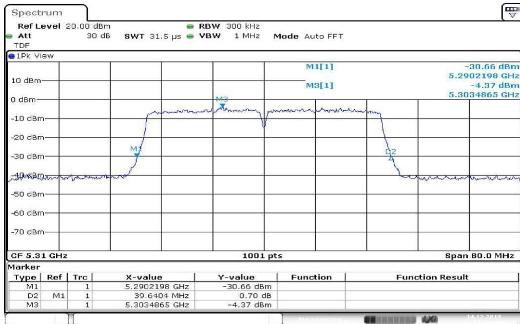
Plot 4: 5310 MHz
