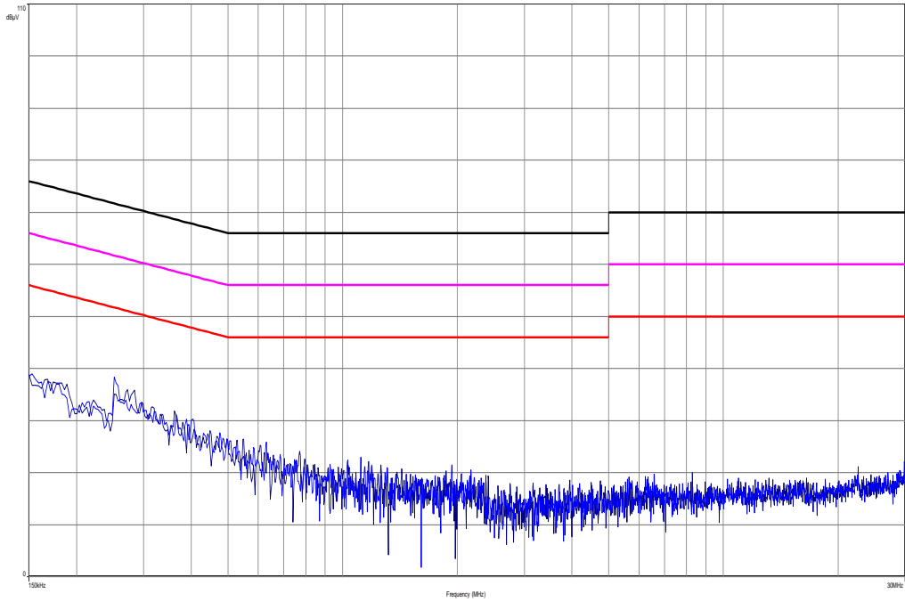
Plot 1: 150 kHz to 30 MHz, phase and neutral line
