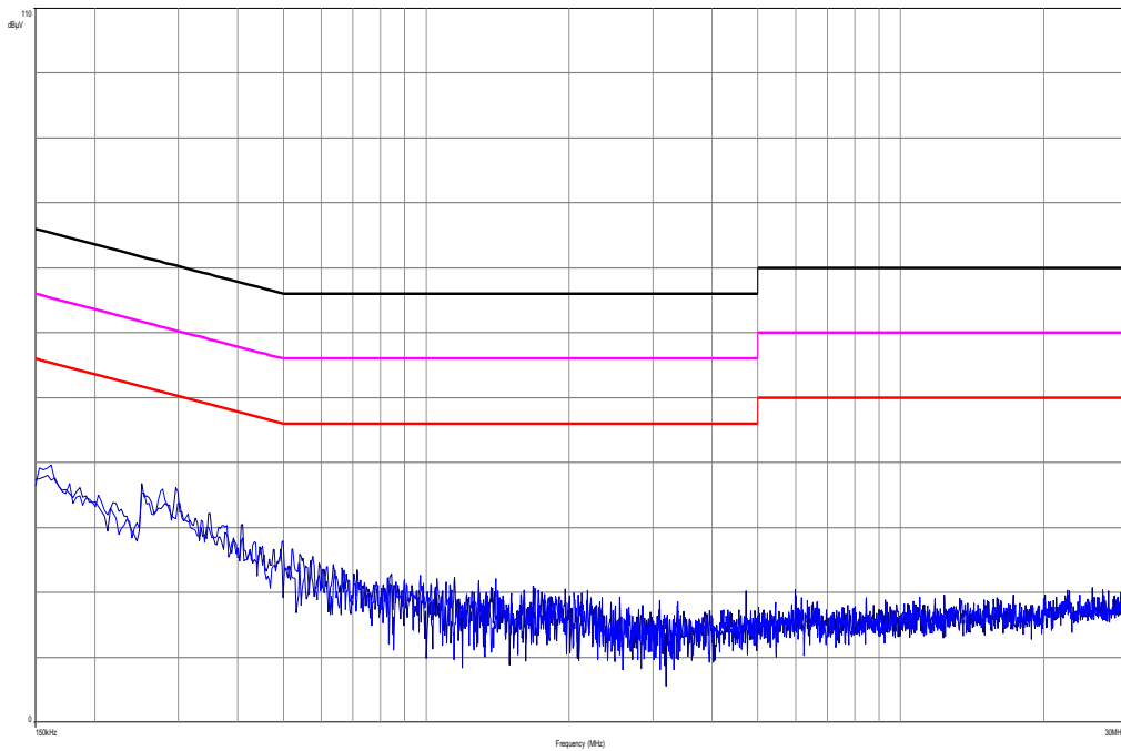
Plot 2: RX mode, 150 kHz to 30 MHz, phase & neutral line
