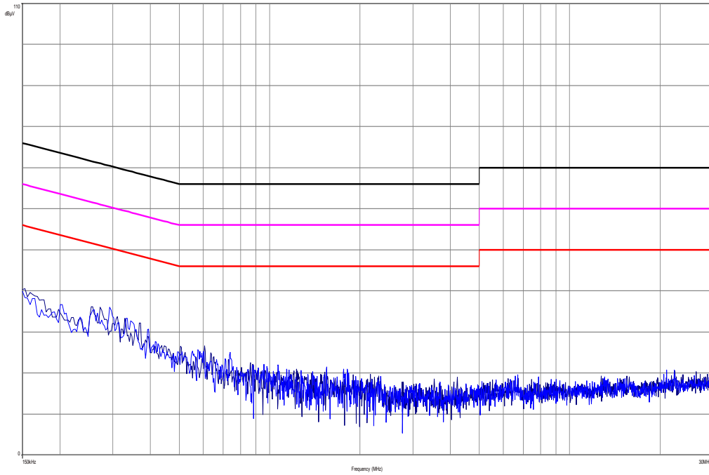
Plot 1: TX mode, 150 kHz to 30 MHz, phase & neutral line
