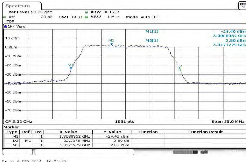
Plot 4: 5320 MHz
