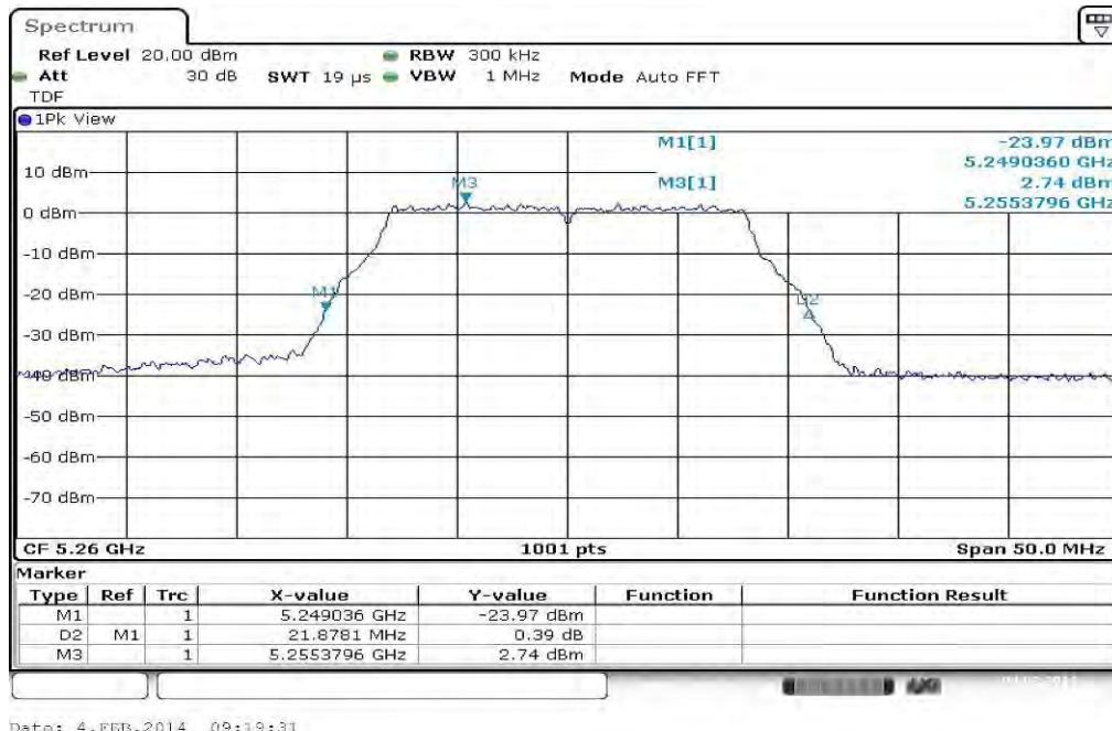
Plot 3: 5260 MHz
