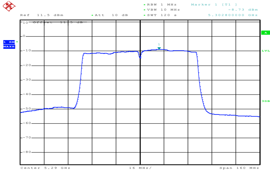
Plot 9: 5290 MHz
