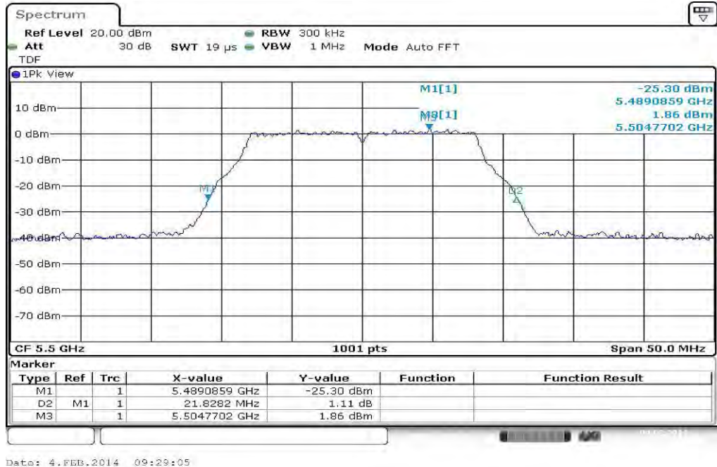
Plot 5: 5500 MHz
