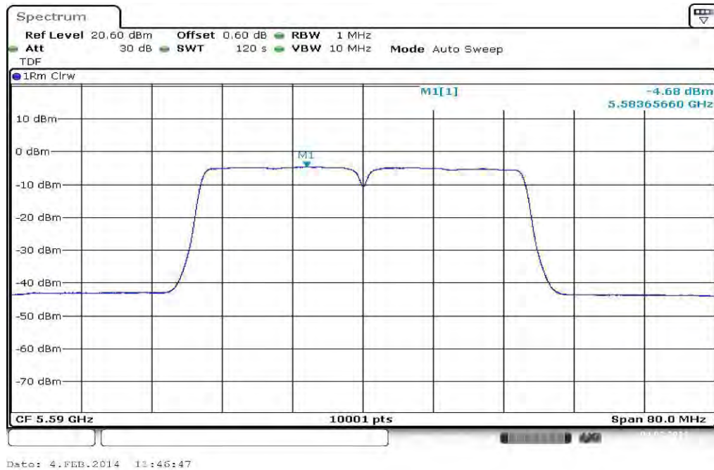
Plot 6: 5590 MHz
