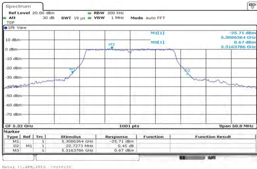
Plot 4: 5320 MHz
