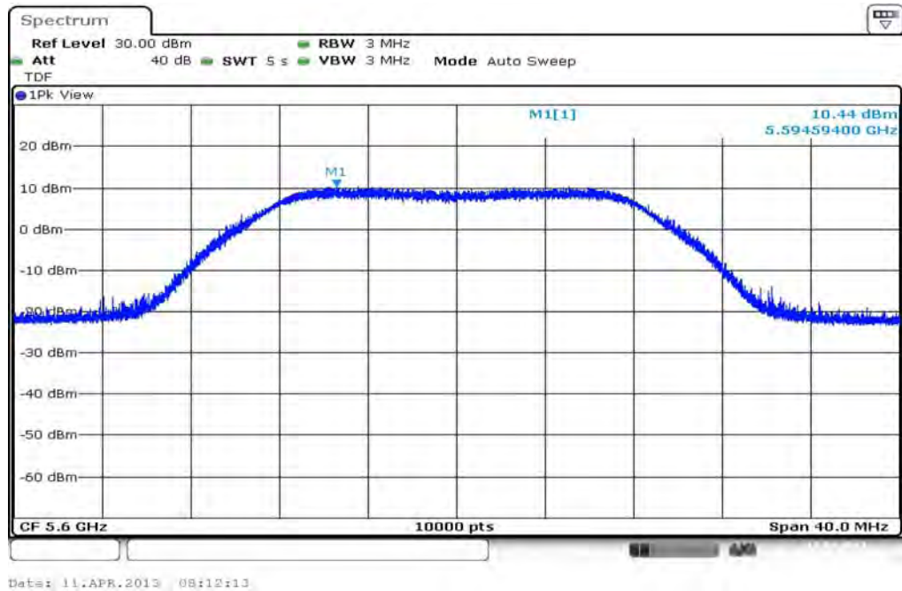
Plot 6: OFDM / a – mode, 5600 MHz
