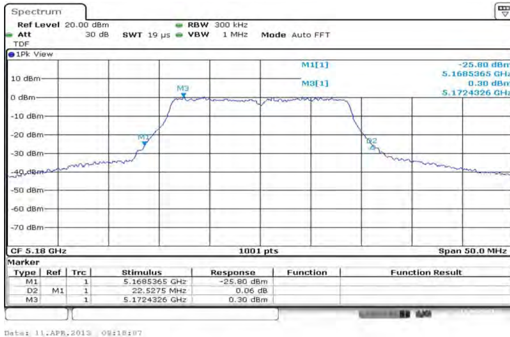
Plot 1: 5180 MHz
