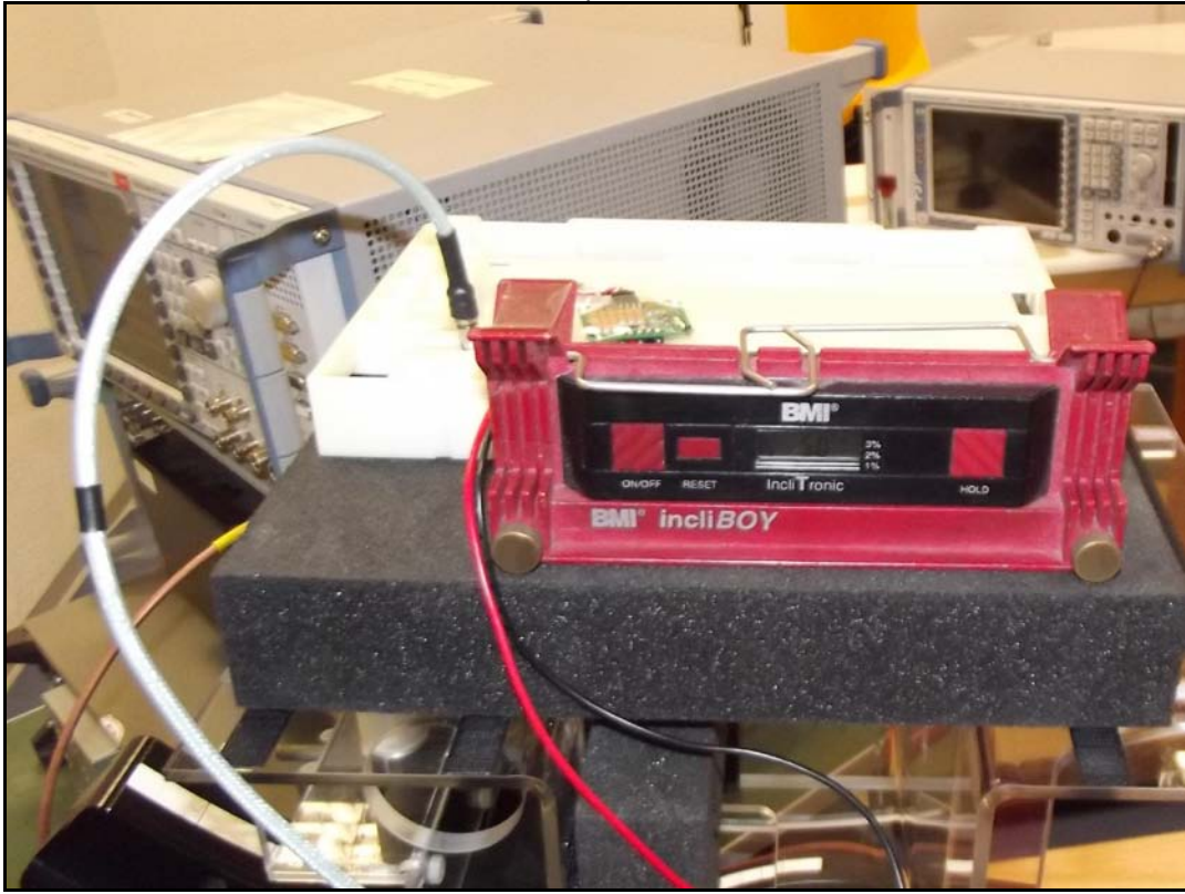
Photo 11: Test of the power back off function
