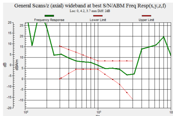
Fig 7.2 GSM1900 Ch661
