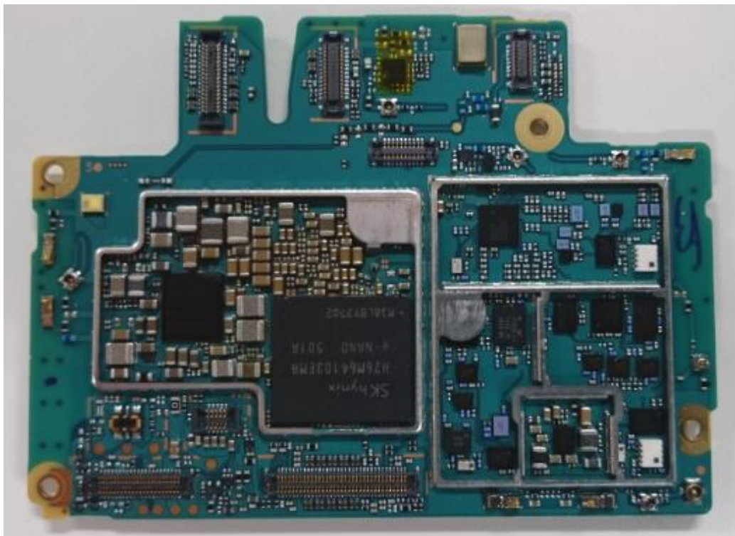
Internal PWB without Shield cases (Rear-side)
