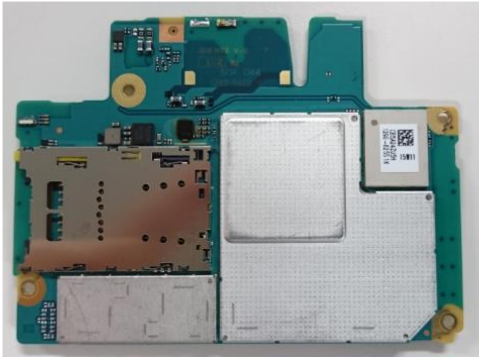
Internal PWB with Shield cases (Front-side)
