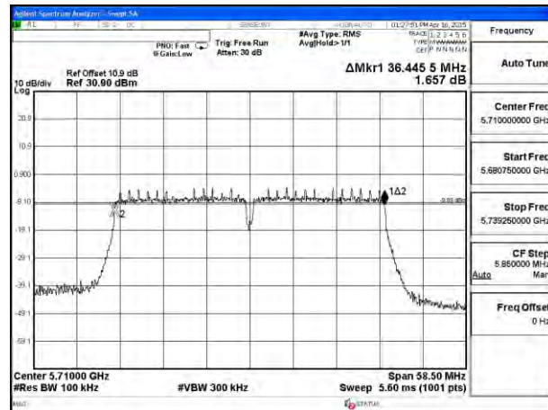
11n HT40 6dB Bandwidth Channel 142
