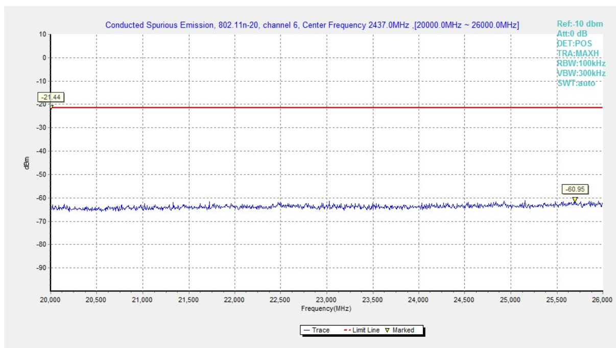
Fig.A.6.1.64 Conducted Spurious Emission (802.11n-HT20, Ch6, 20 GHz-26 GHz)
