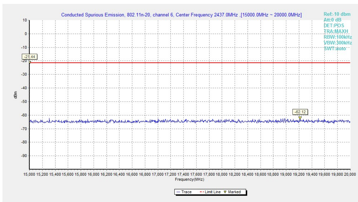
Fig.A.6.1.63 Conducted Spurious Emission (802.11n-HT20, Ch6, 15 GHz-20 GHz)
