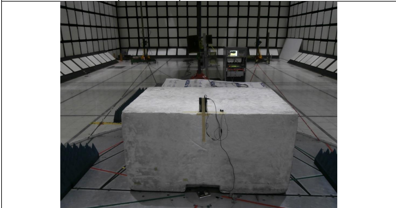
RADIATED BACK PHOTO (ABOVE 1 GHz)
