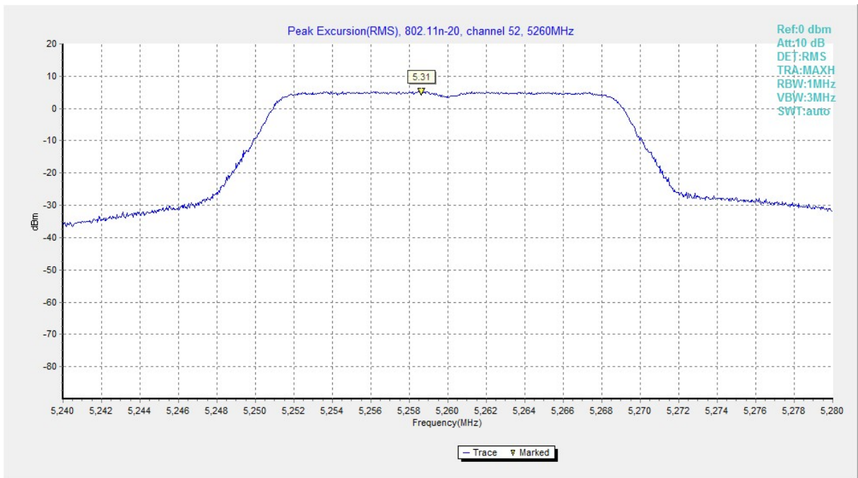
Fig. 167 Peak Excursions (802.11n-HT20, ch52, average)
