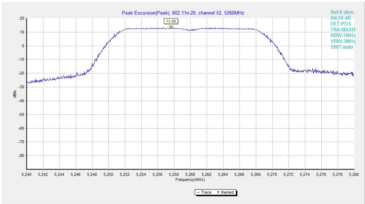
Fig. 164 Peak Excursions (802.11n-HT20, ch52, peak)
