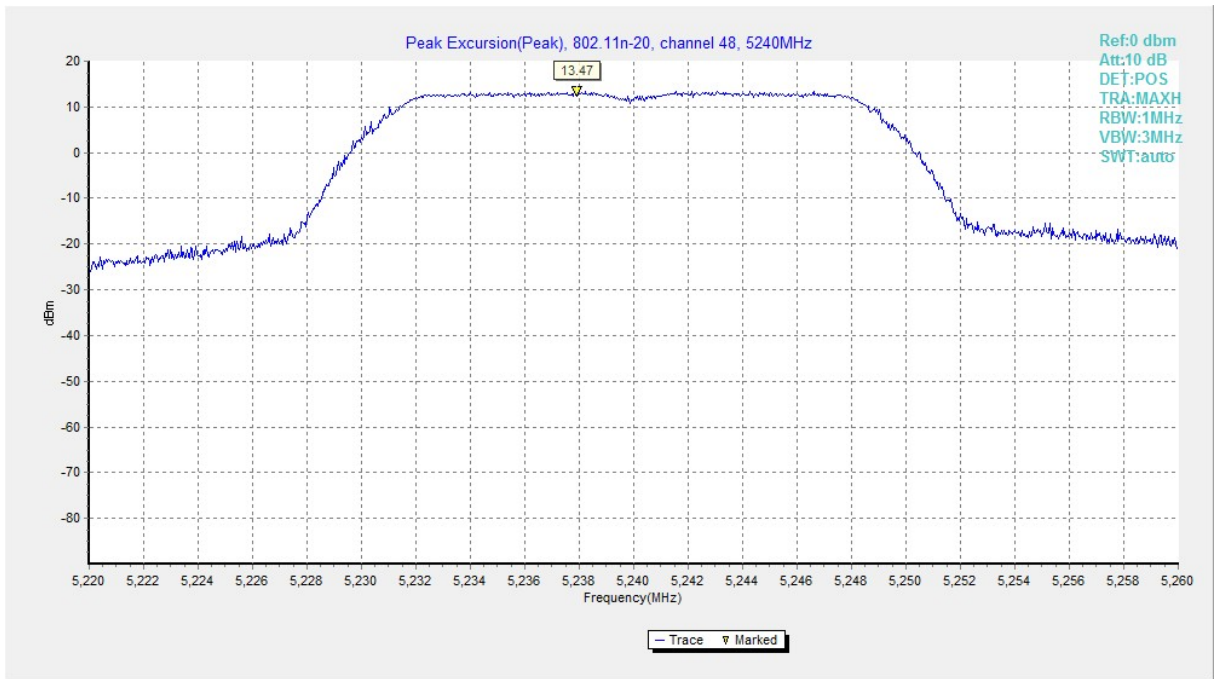
Fig. 160 Peak Excursions (802.11n-HT20, ch48, peak)
