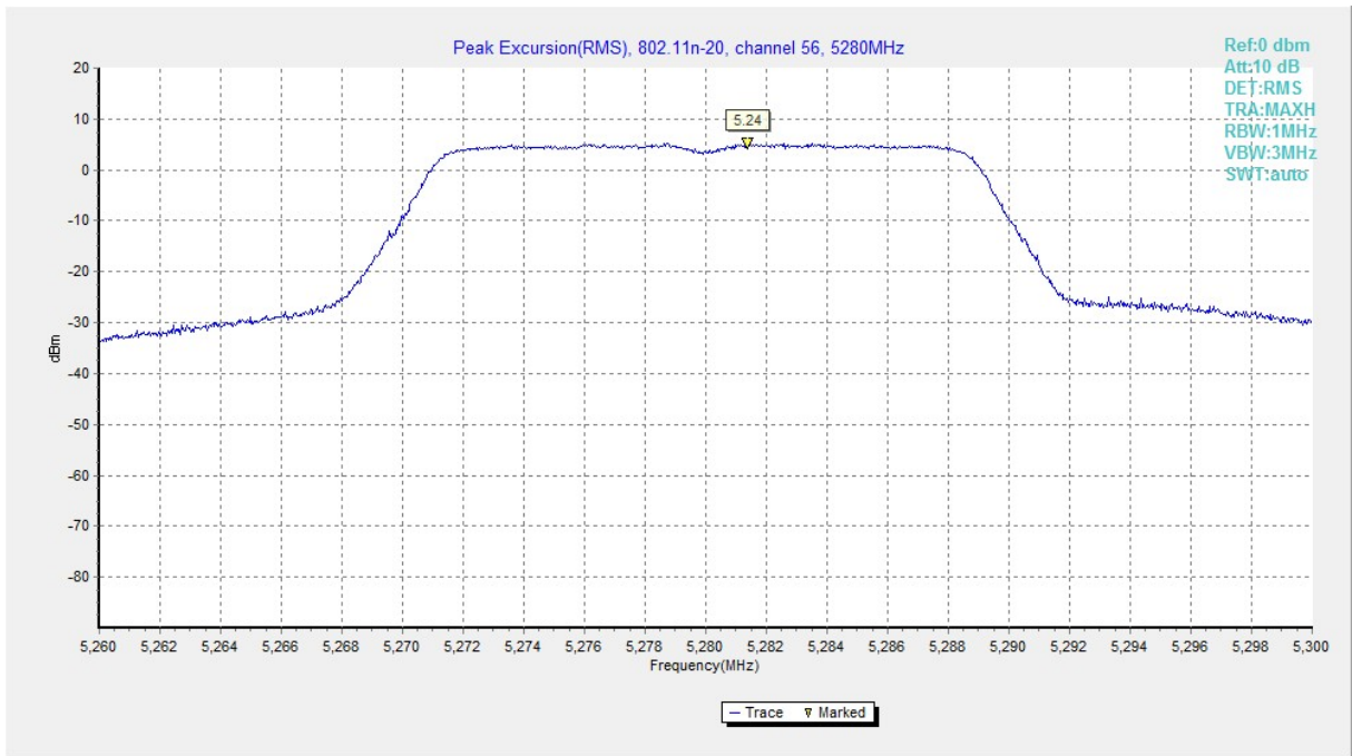
Fig. 168 Peak Excursions (802.11n-HT20, ch56, average)
