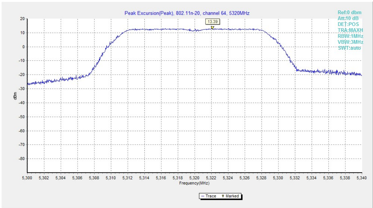
Fig. 166 Peak Excursions (802.11n-HT20, ch64, peak)
