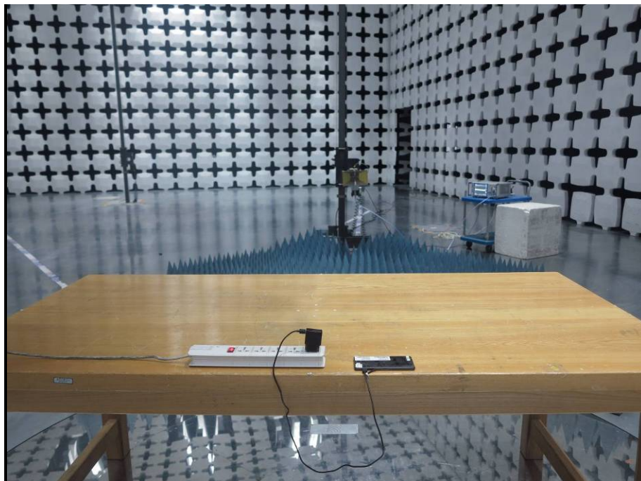
Picture C-12: Radiated Spurious Emission(PART15C)
