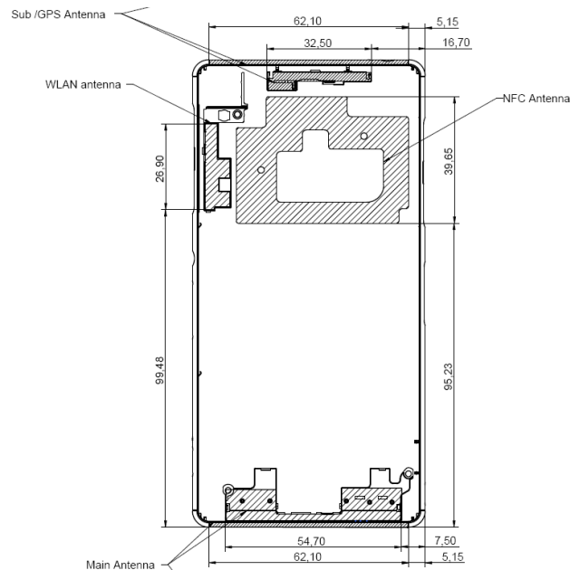
Antenna positioning diagram with separation distance
