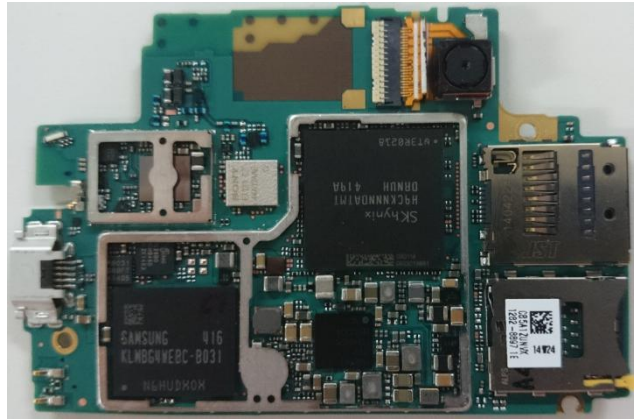
Internal PWB without Shield cases (Front-side)
