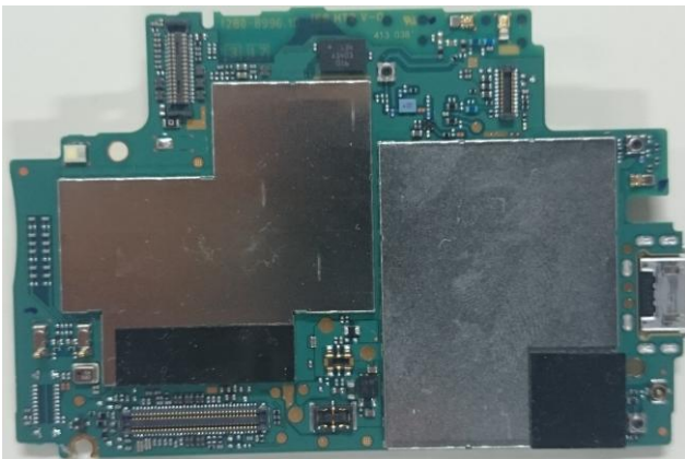
Internal PWB with Shield cases (Rear-side)
