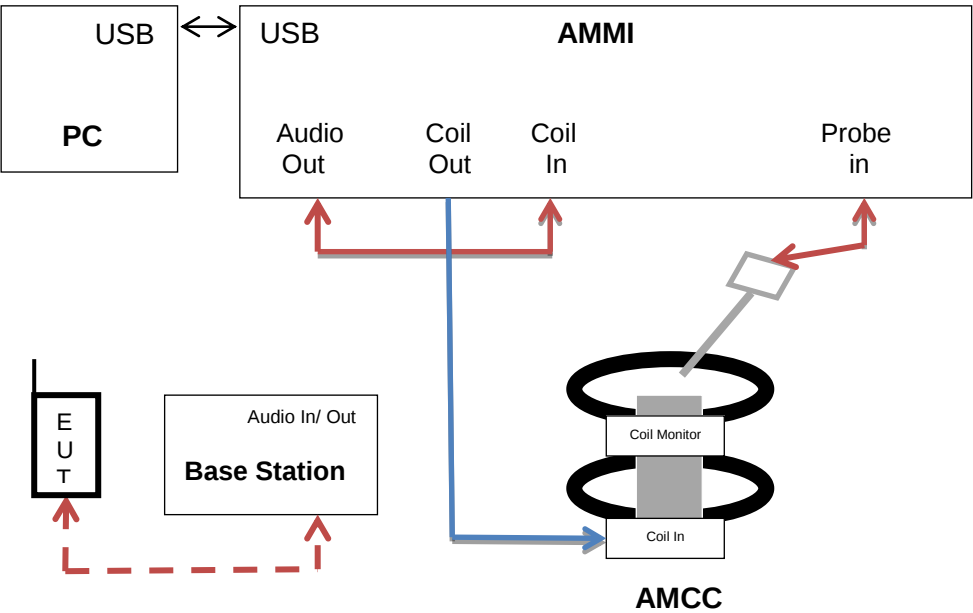
Figure 3: Signal from AMMI to CMU200 measurement Set-up
