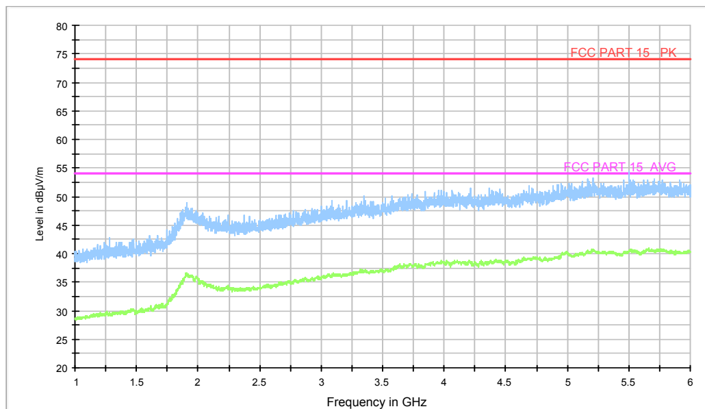
Normal RE_1G-6GHz
