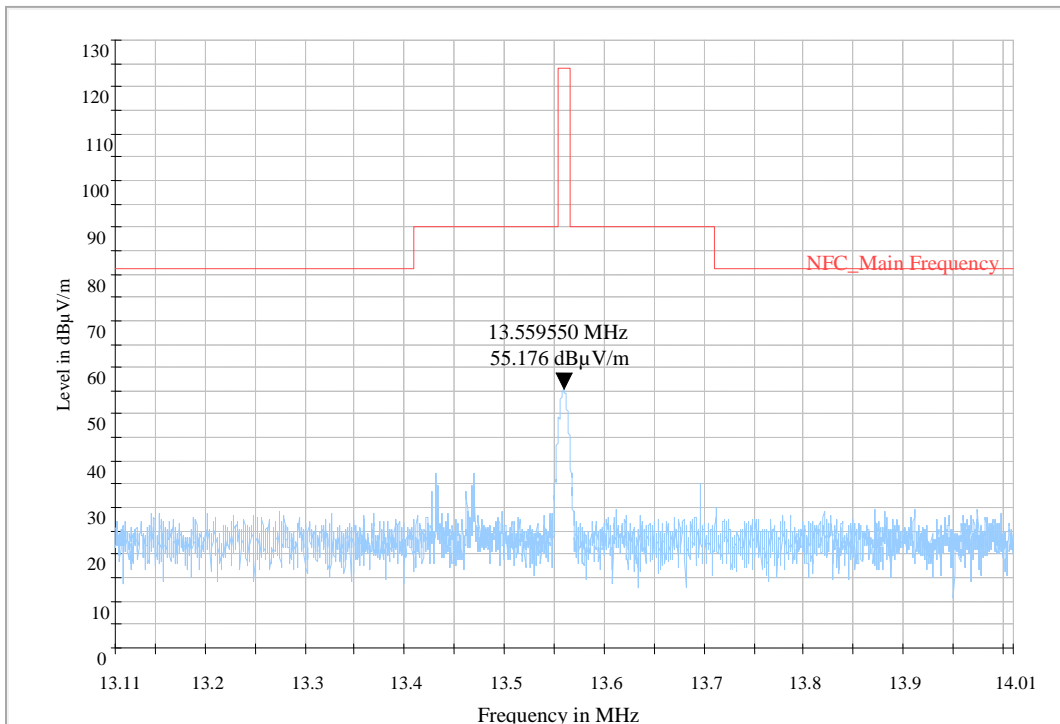
RE_NFC Main Frequency_13.110MHz-14.010MHz
