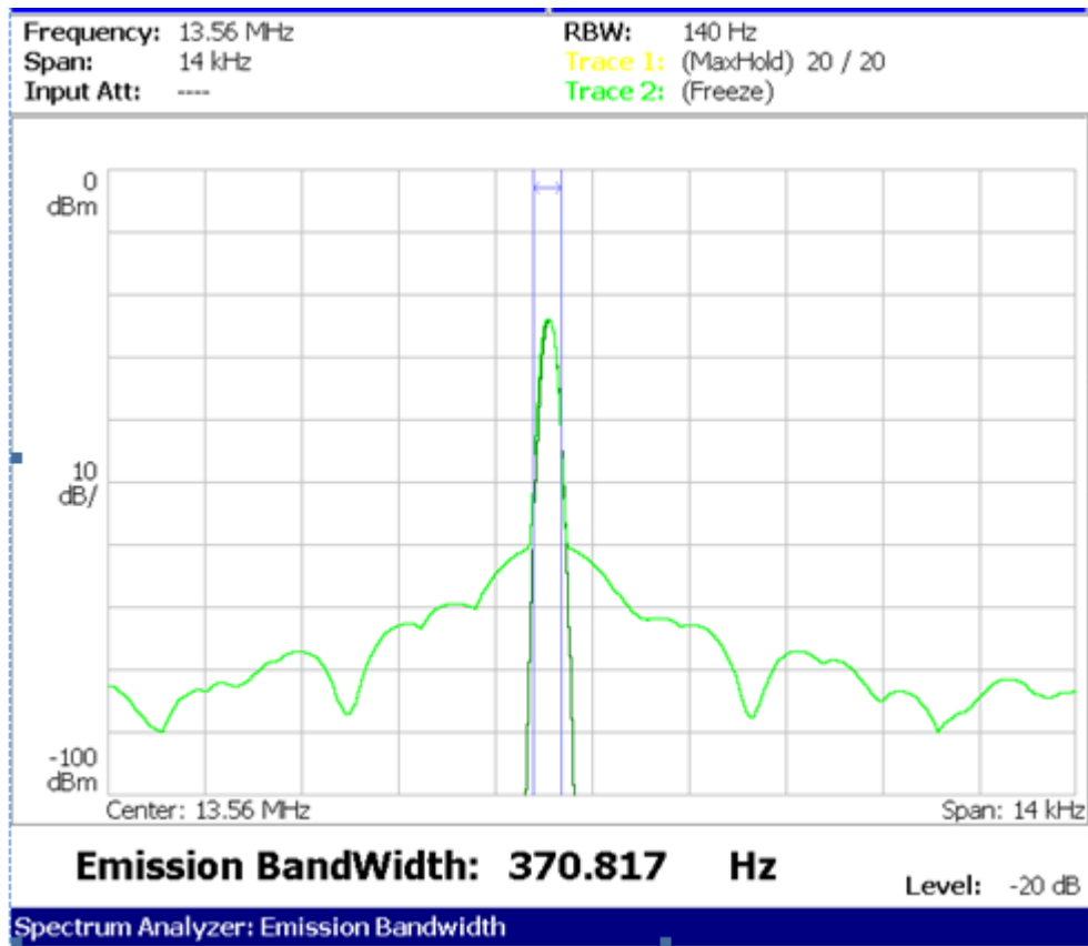
Figure A-4: 20dB Bandwidth Test result
