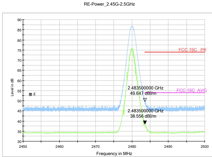
Fig.17. Radiated emission (Power): High Channel
