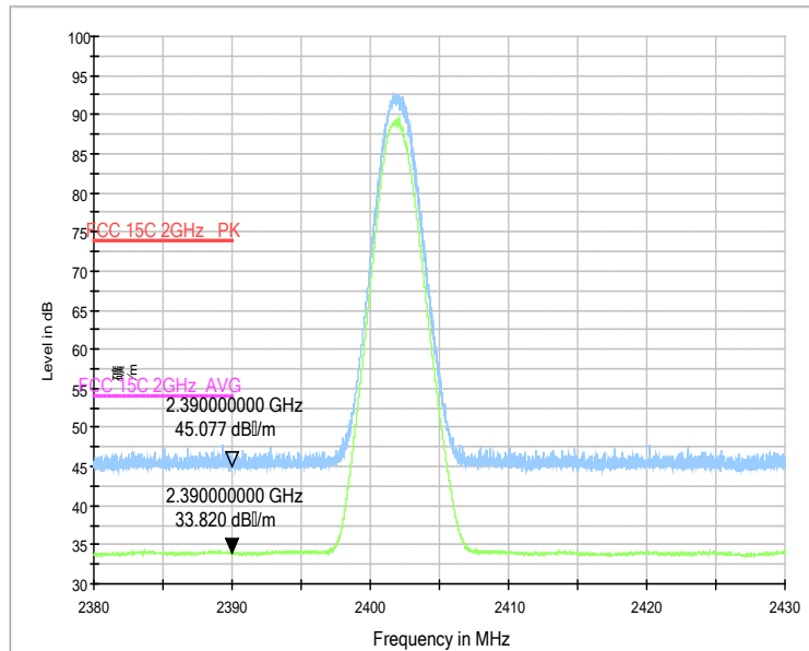
RE-Power_2.38G-2.43GHz
