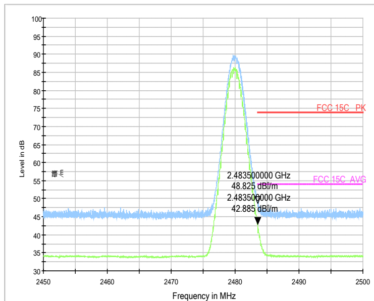
RE-Power_2.45G-2.5GHz
