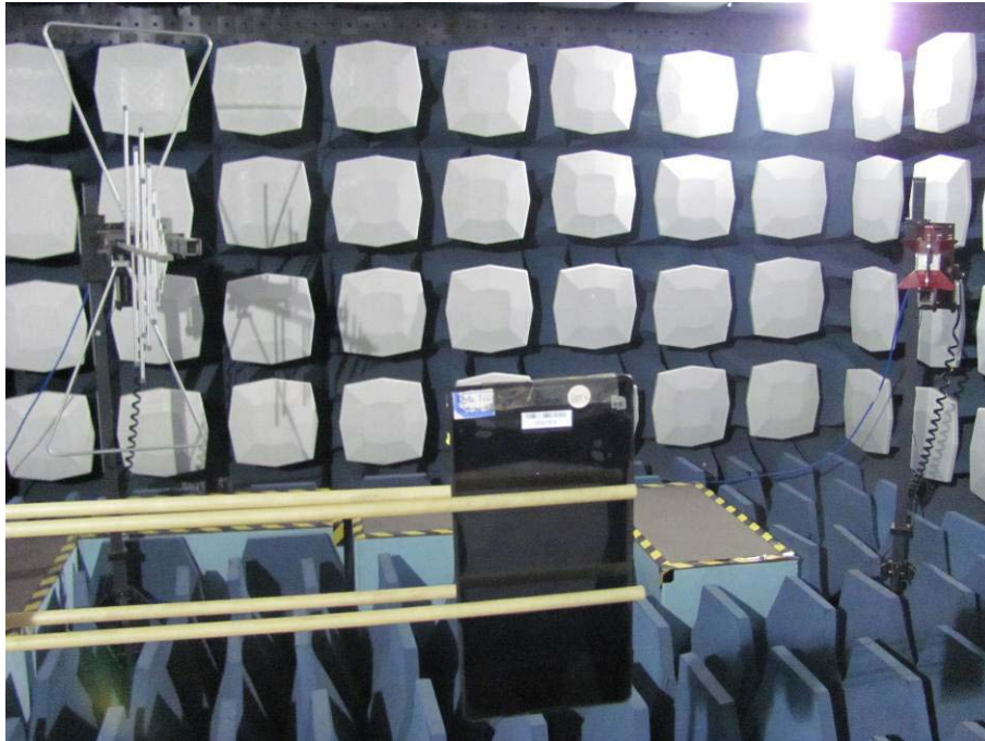
Picture-1: Pic.1 Radiated spurious emission
