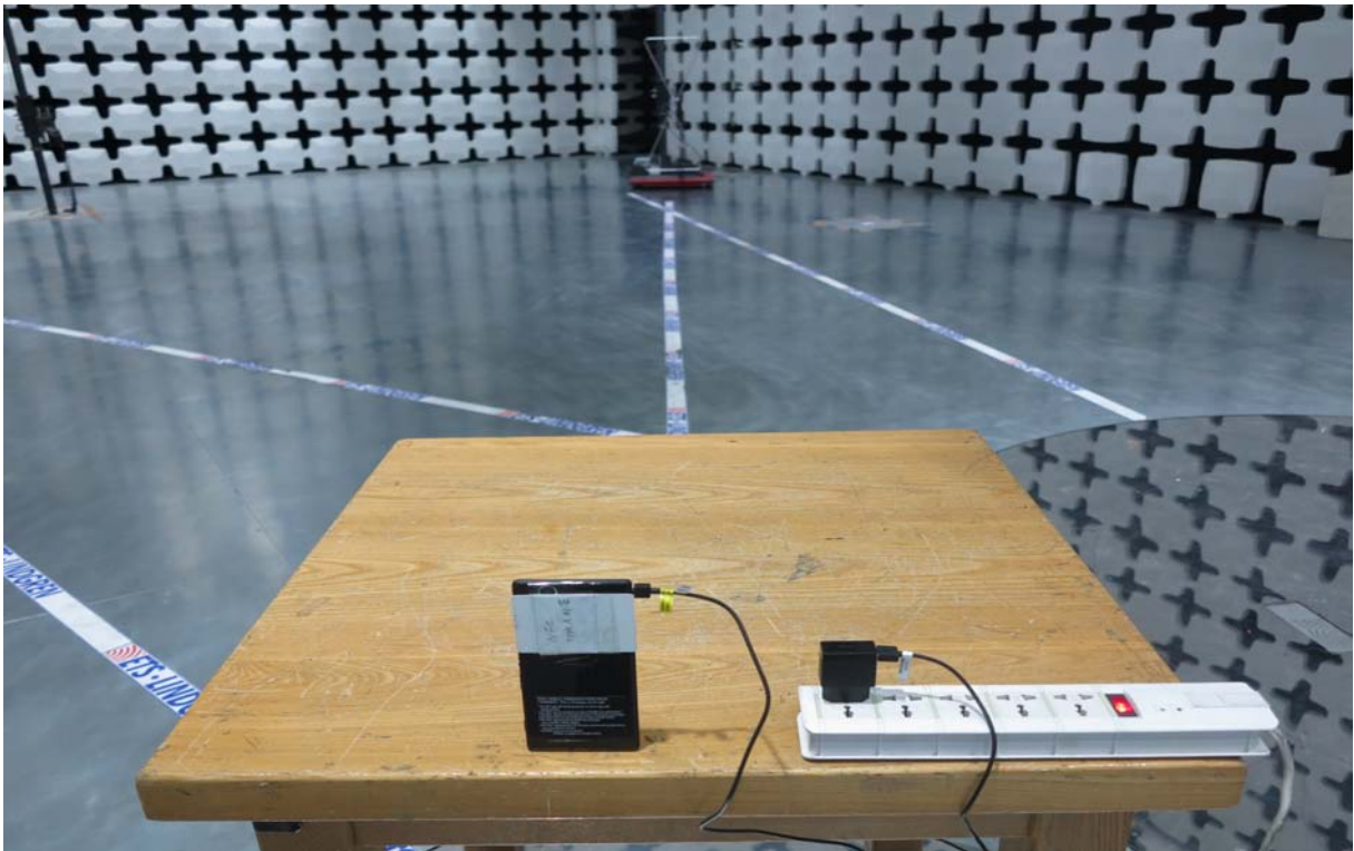
Picture-4: Field Strength Measurements (Above 30MHz) for Par15C_NFC
