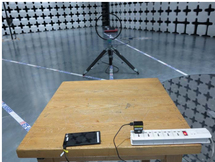
Picture-6: Radiated emission for Part15C
