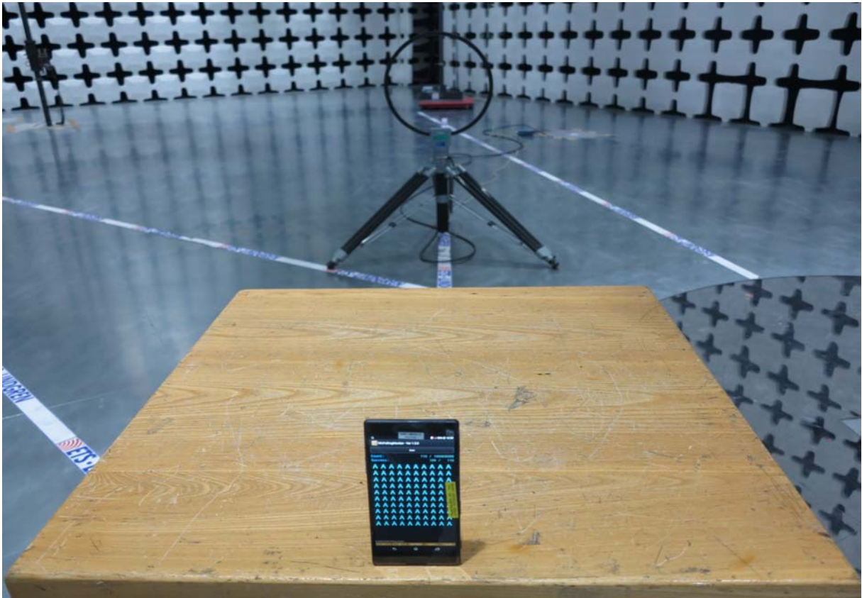
Picture-3: Field Strength Measurements (Below 30MHz) for Par15C_NFC
