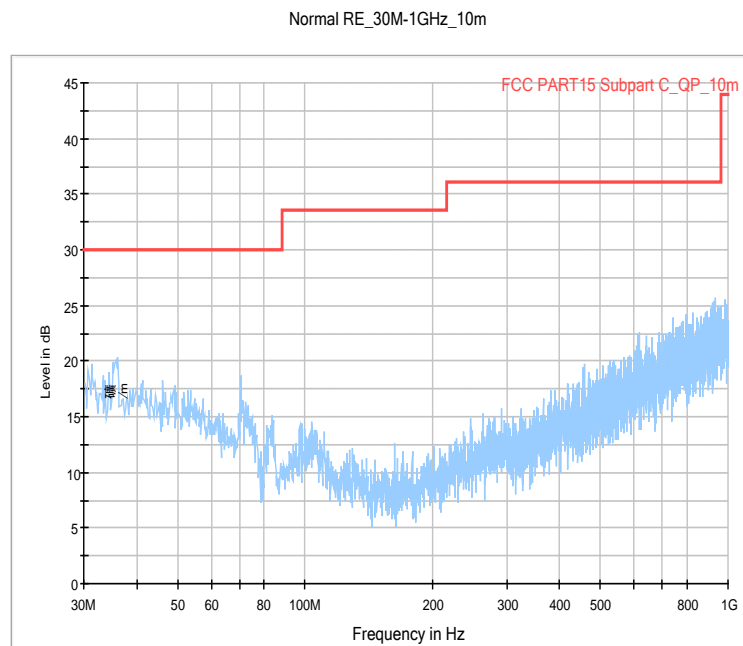
Fig.24. Radiated emission: GFSK, 2480MHz, 30 MHz - 1 GHz
