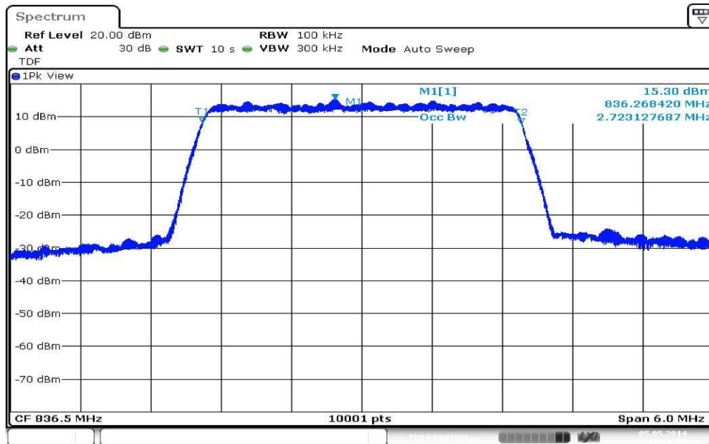
Plot 3: 3 MHz (99% - OBW)
