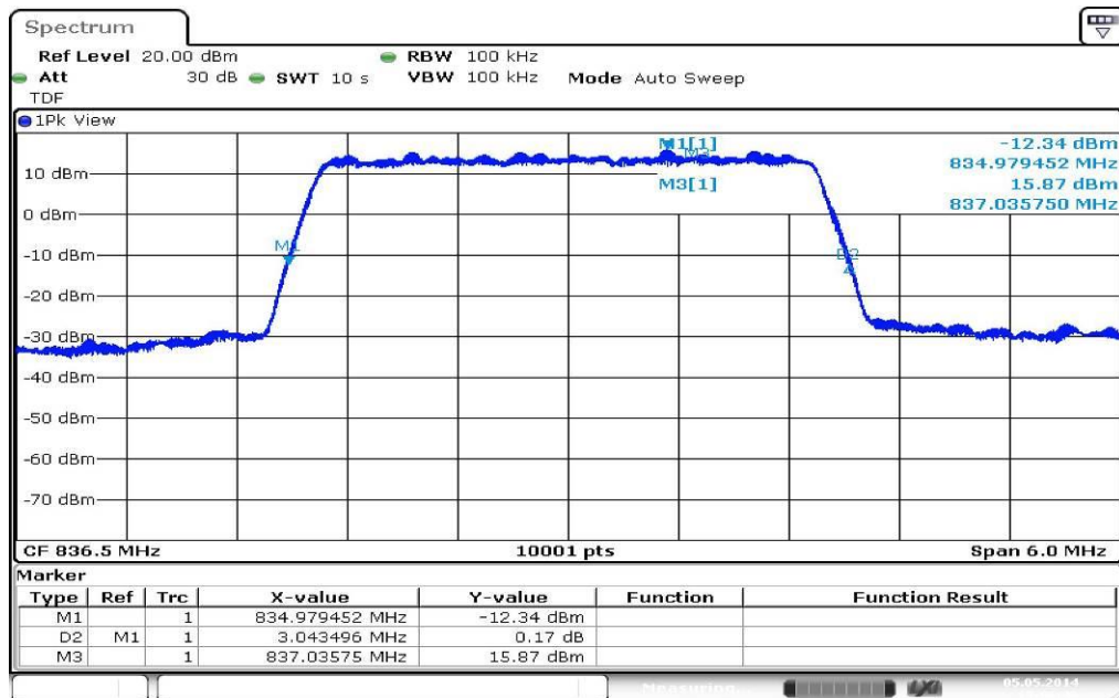
Plot 4: 3 MHz (-26 dBc BW)
