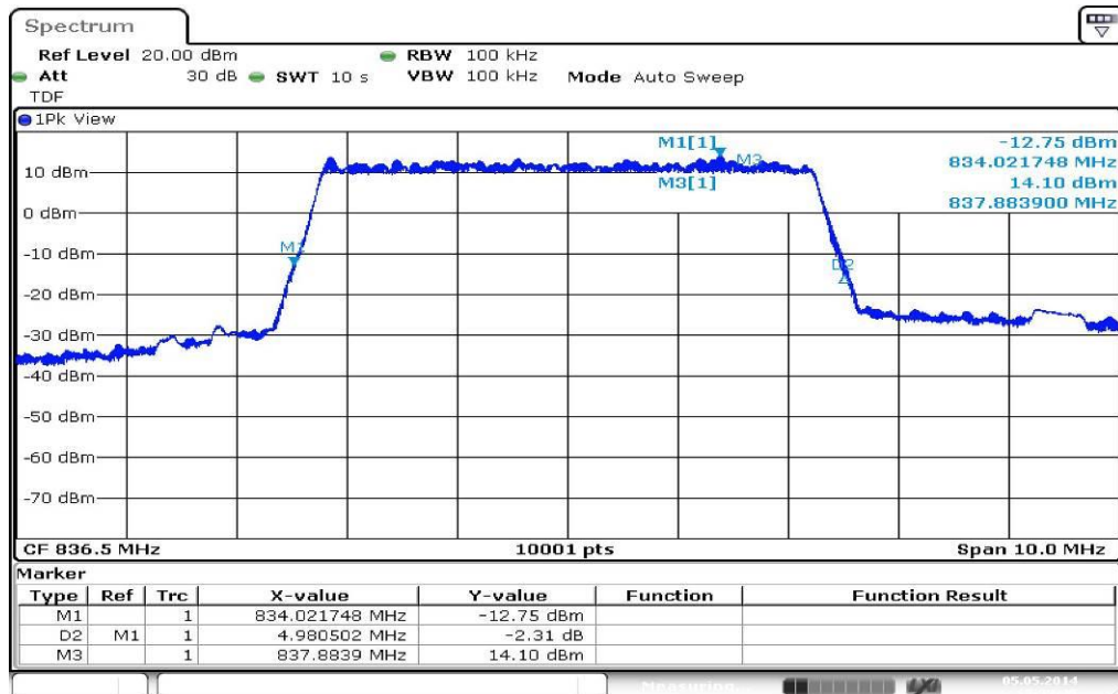
Plot 6: 5 MHz (-26 dBc BW)
