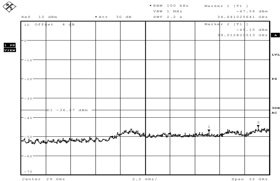
Plot 2: TX mode, mid channel, 18 GHz to 40 GHz
