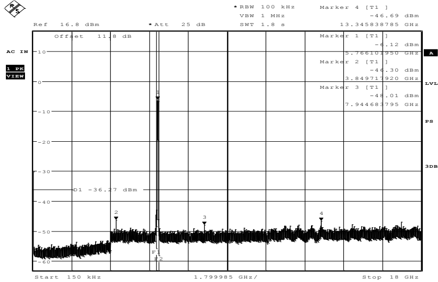
Plot 1: TX mode, mid channel, up to 18 GHz
