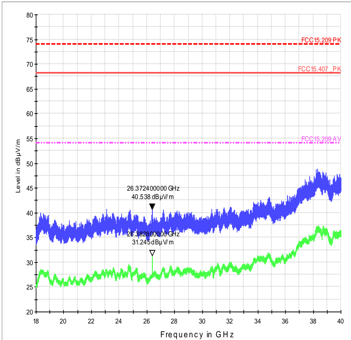
EMI Scan_18_40GHz_Pre
