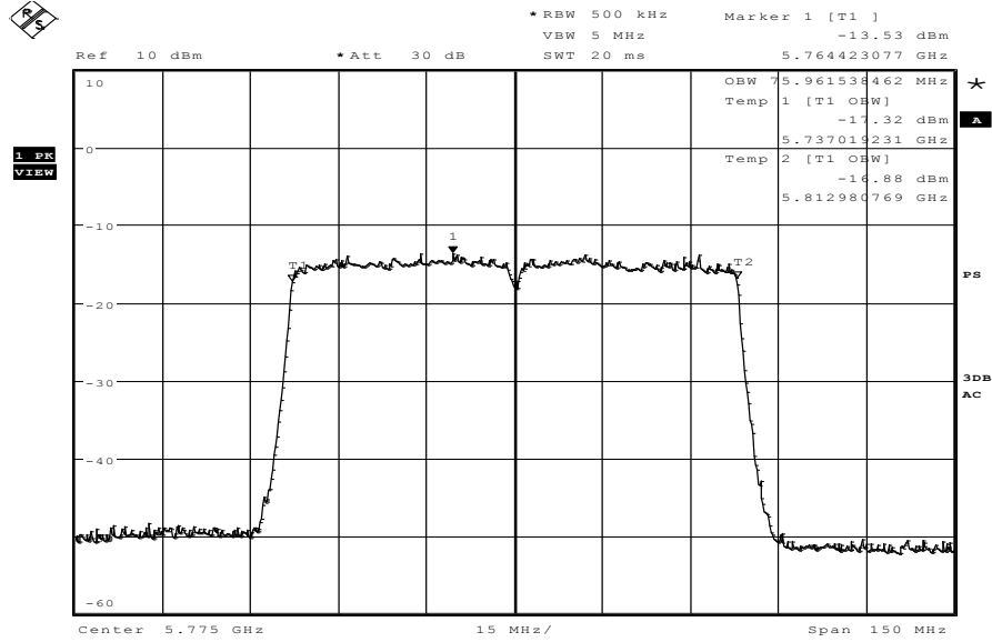
Plot 1: TX mode, mid channel
