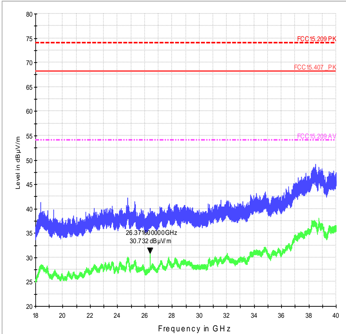
EMI Scan_18_40GHz_Pre
