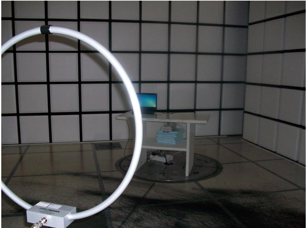
9kHz- 30MHz Measurement setup: EUT+Notebook Mode of test
