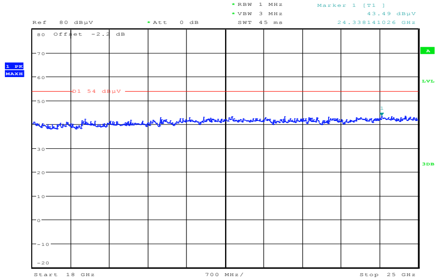
Plot 8: 18 GHz to 25 GHz, mid channel, vertical & horizontal polarization – valid for all channels
