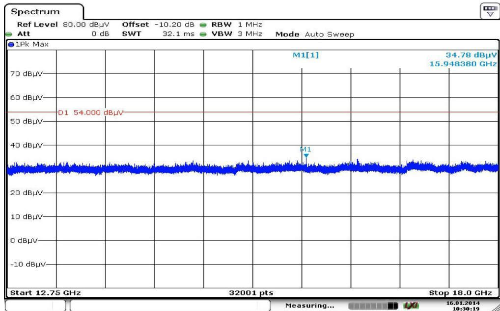
Plot 23: 12 GHz to 18 GHz, 5500 MHz, vertical & horizontal polarization
