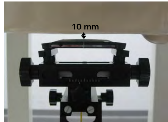
Fig.12 EUT back to flat phantom
