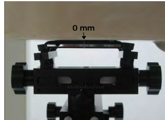
Fig.18 EUT back to flat phantom
