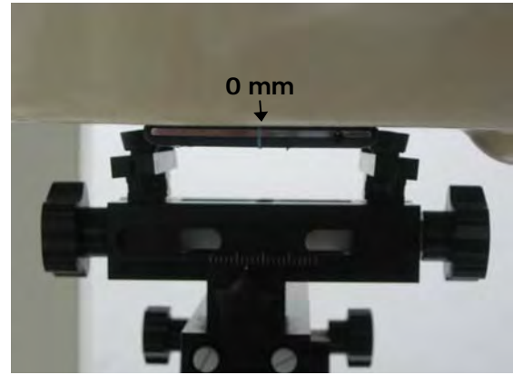
Fig.17 EUT front to flat phantom
