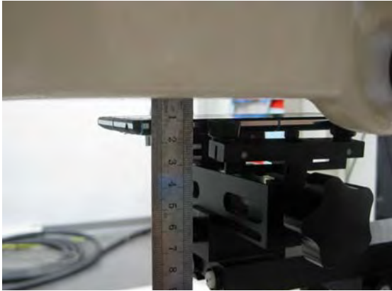
Fig.11 EUT front to flat phantom
