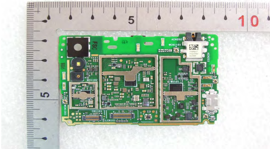
BT/WLAN/Diversity/GPS Antenna
