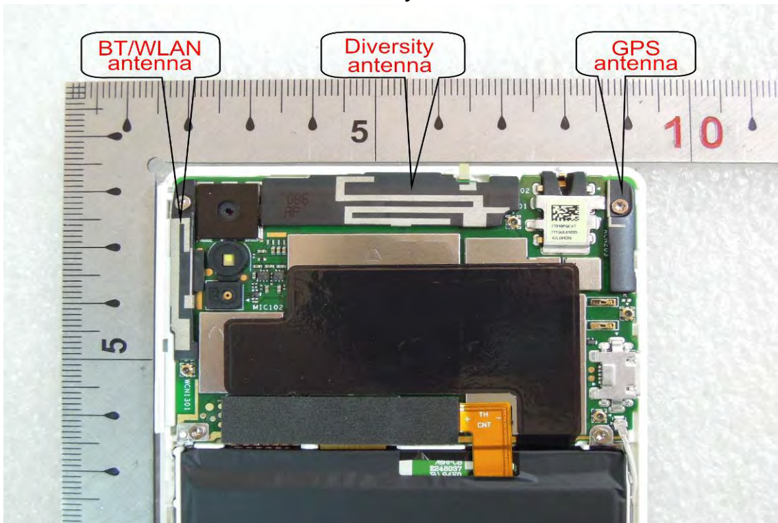
BT/WLAN/Diversity/GPS Antenna
