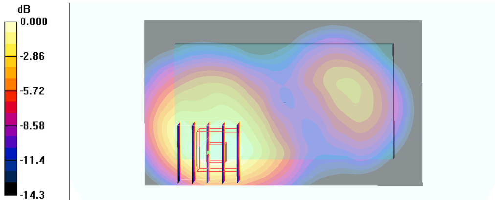
0 dB = 1.64mW/g
