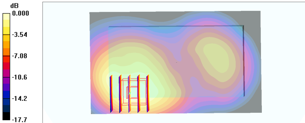
0 dB = 0.901mW/g
