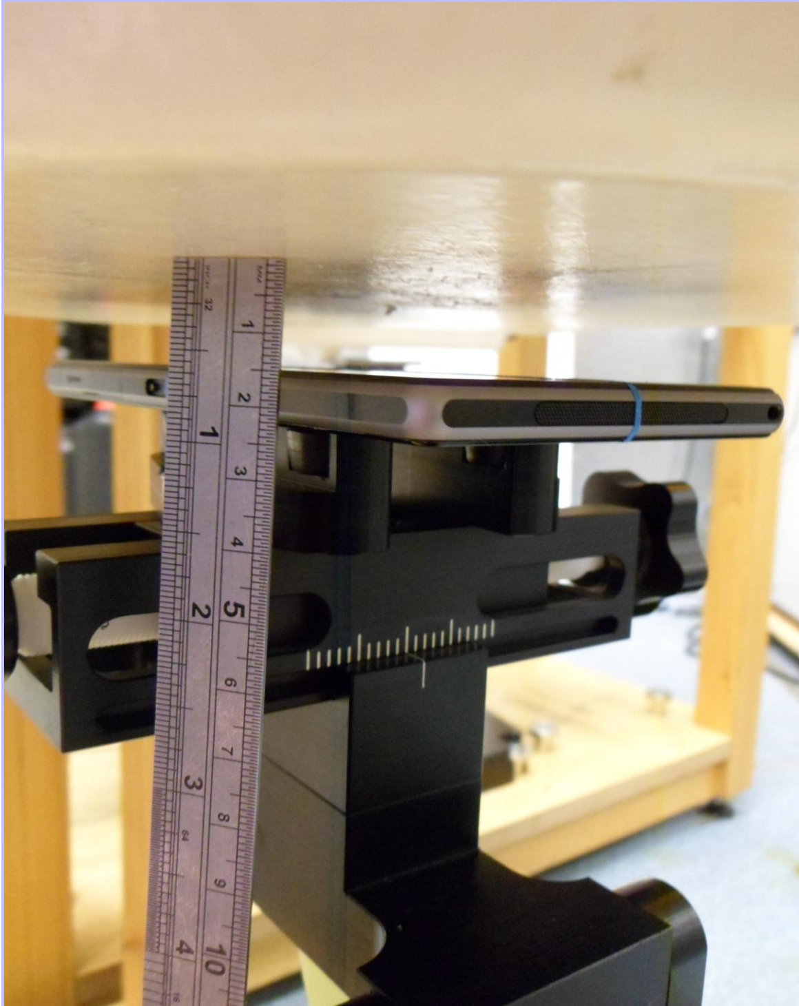
PHT/10014948JD25/007: Front of EUT Facing Phantom at 15mm
