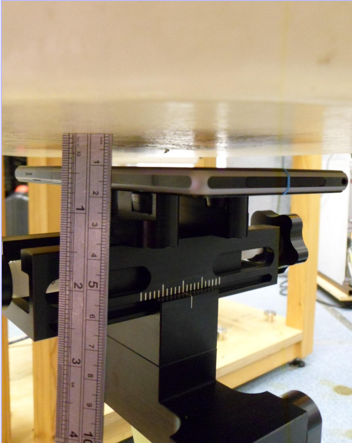
PHT/10014948JD25/006: Front of EUT Facing Phantom at 10mm
