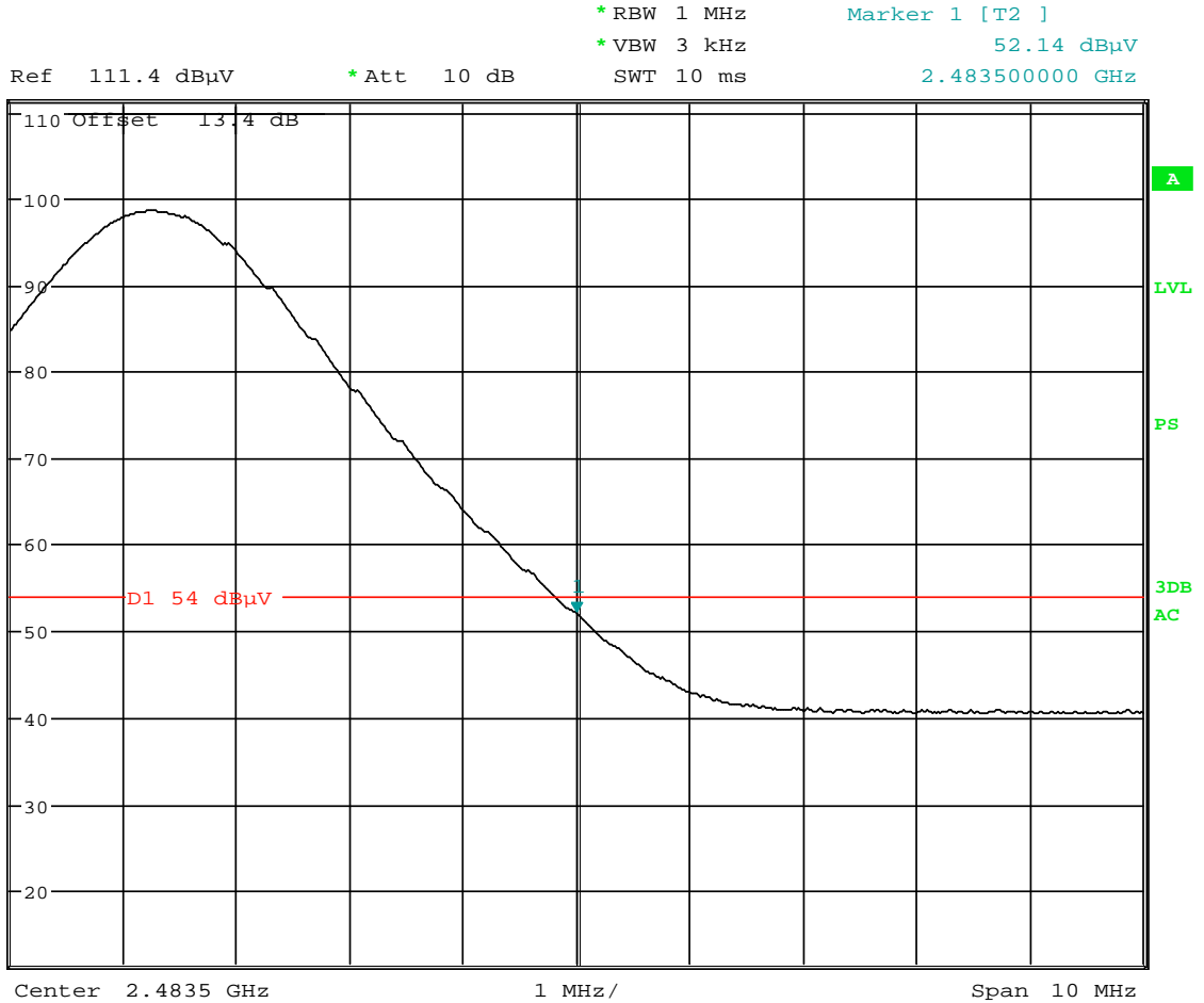
Plot 6-18.Radiated Restricted Band Edge Plot (Average)
