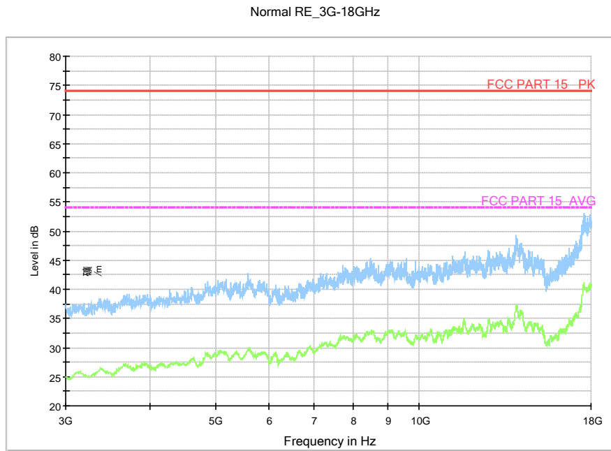
Fig.9. Radiated emission: Channel 39, 3 GHz - 18 GHz
