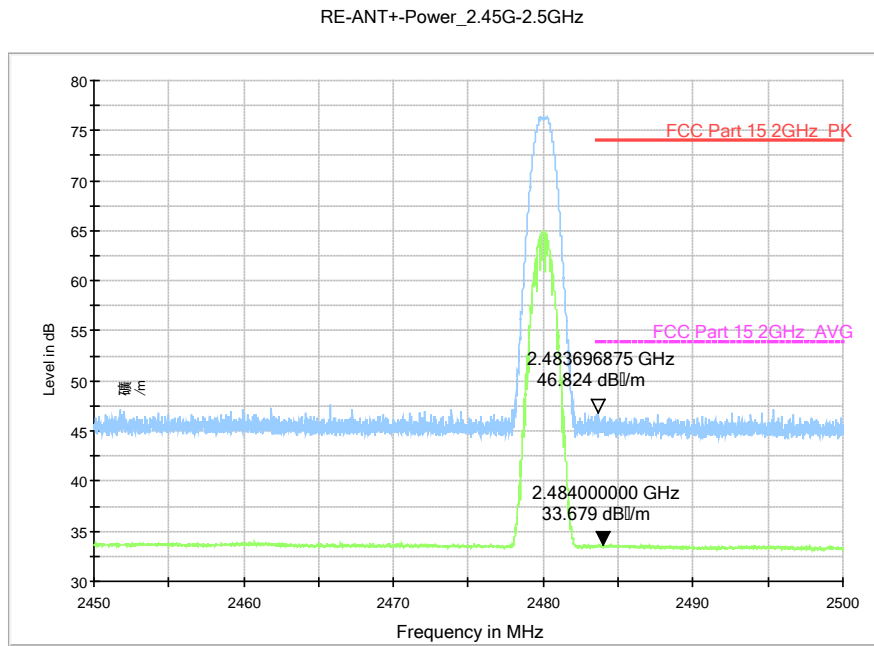
Fig.15. Radiated emission (Power): High Channel
