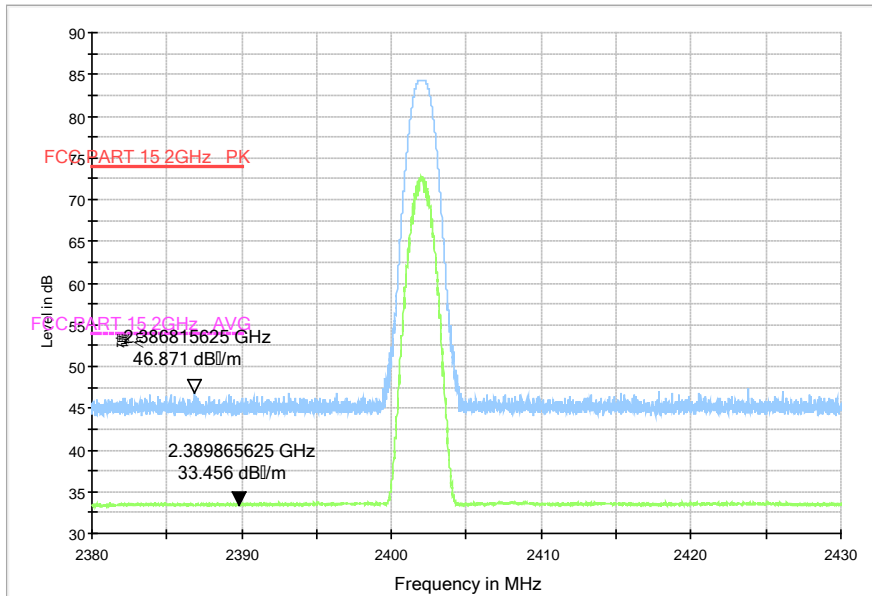
RE-ANT+-Power_2.38G-2.43GHz
