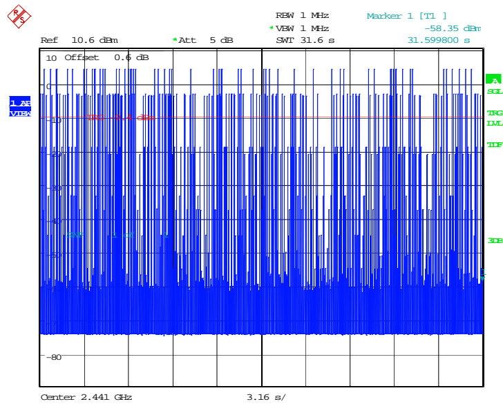
Fig.92. Time of occupancy (Dwell Time): Channel 39, GFSK-DH5
